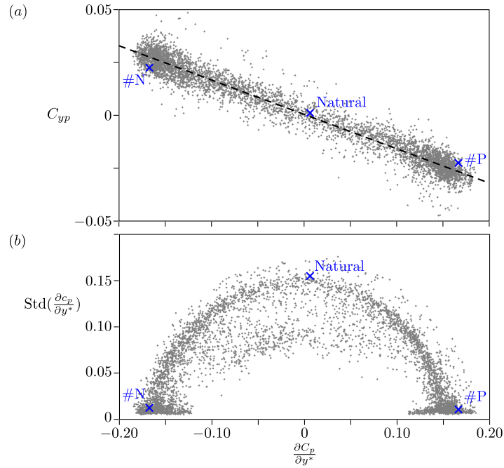
Figure 7.4. Scatter plots of C_{yp} vs. \partial C_p/\partial y^* (a) and of \text{Std}(\partial C_p/\partial y^*) vs. \partial C_p/\partial y^* (b) for the vertical cylinder positions x_C^* > 0.2 . The dashed line is the linear fit C_{yp} = -0.16 \partial C_p/\partial y^* . The crosses are the natural values.
