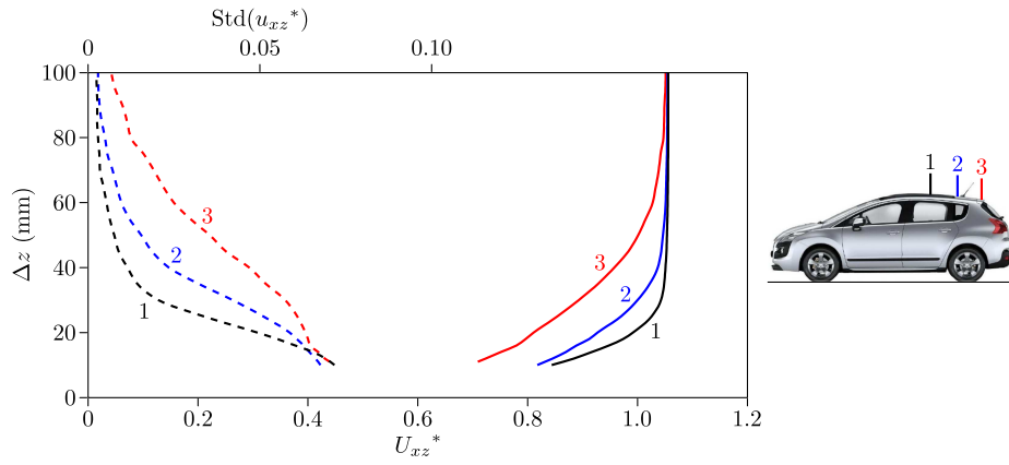
Figure 10.3. Mean (continuous lines) and fluctuating (dashed lines) velocity profiles of the boundary layer on the roof of the Peugeot 3008 in the plane y = 0.12 m: \Delta x = -1.0 m, black lines; \Delta x = -0.5 m, blue lines; \Delta x = -0.05 m, red lines. \Delta x and \Delta z are the algebraic distances to the roof end and to the roof surface respectively.
