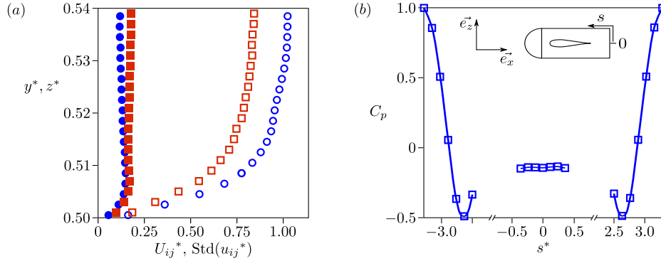
Figure 3.2. (a) Mean and fluctuating velocity profiles (empty and filled symbols respectively) of the boundary layer at the trailing edge: \circ , u_{xz} in the plane y^* = 0 ; \square , u_{xy} in the plane z^* = 0 . (b) Pressure distribution on the body in the plane y^* = 0 .
