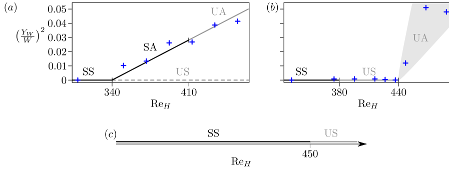
Figure 4.6. Bifurcation scenarii of the wake for C^* = 0.06 (a), C^* = 0.04 (b) and C^* = 0.02 (c): +, experimental data; the black and gray lines are steady and unsteady regimes respectively; the continuous and dashed lines are stable and unstable regimes respectively.
