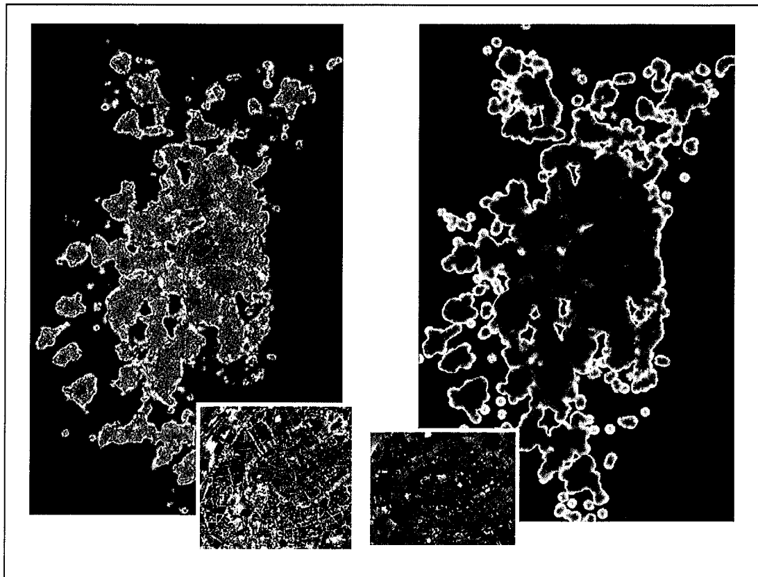
Fig. 2: Images of the Gravelius (left) and Miller (right) indicators for the city of Strasbourg. Images at bottom display zooms of the city center for each indicator.
