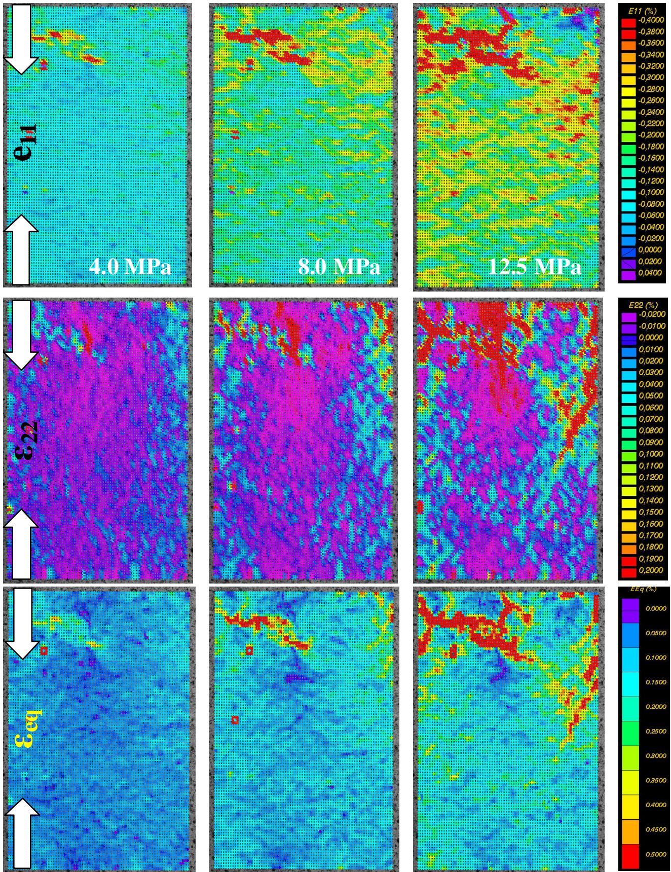
Fig. 13. In-plane strain components \varepsilon_{11} , \varepsilon_{22} and \varepsilon_{eq} maps for 6RAT sample, at loading stages 4.0, 8.0 and 12.5 MPa reported in the Fig. 10. Grid size = 2813 x 4583 pixels. Measurements basis of 56 pixels = 424 \mu\text{m} .
