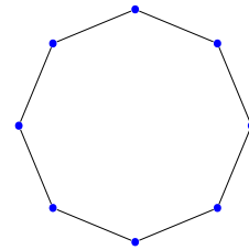
FIGURE 1.4 – C_8
