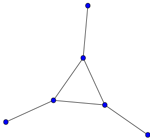
FIGURE 4.4 – G_6^1
