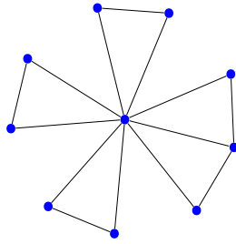
FIGURE 4.18 – F_{10,14}
