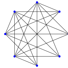
FIGURE 1.7 – K_{4,2,2}
