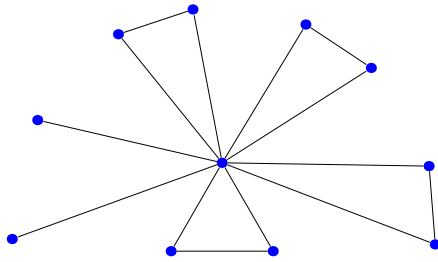
FIGURE 4.16 – B_{4,3}
