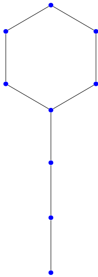
FIGURE 3.3 – Lol_{9,6}
