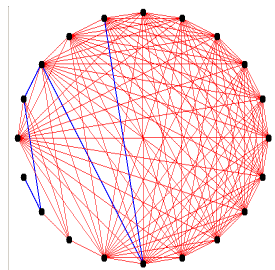
FIGURE 1.15 – G_D^{heur}
