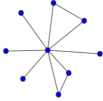
FIGURE 4.2 – B_{2,4}
