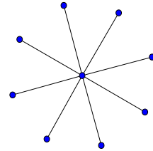
FIGURE 1.2 – S_9
