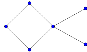
FIGURE 4.6 – G_6^3
