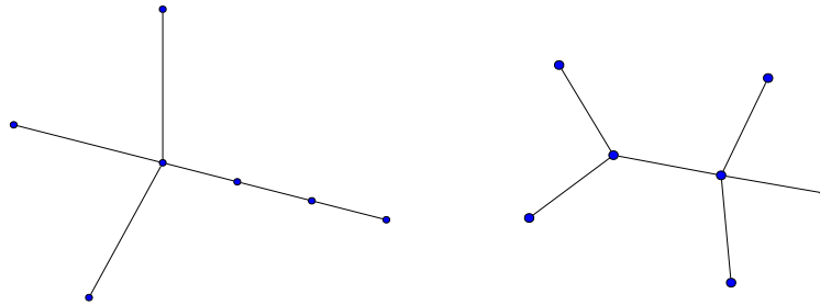
FIGURE 4.10 – S_5^1, S_5^2
