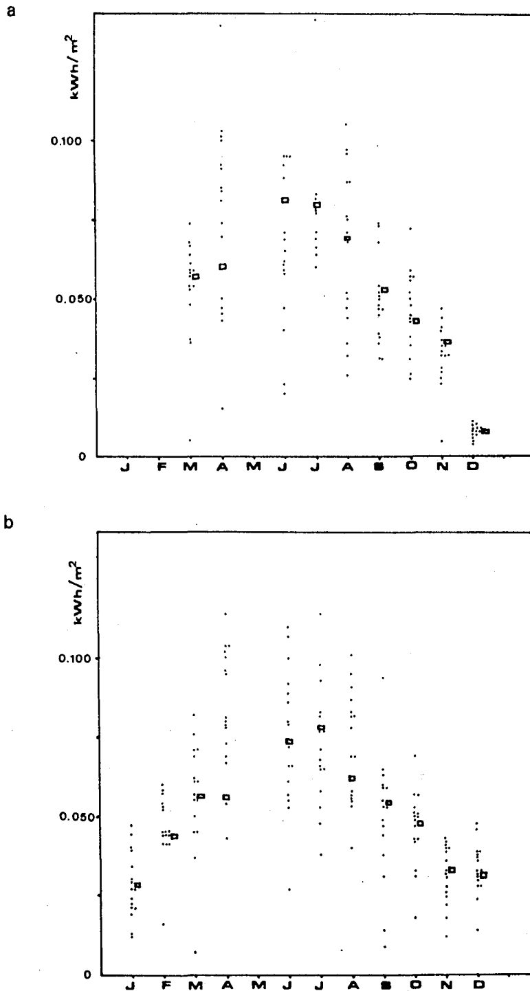
FIGURE 2 Variation of the r.m.s. error versus month for each station. The square means all stations merged together. a) 9.10 h UT; b) 12-13 h UT.
