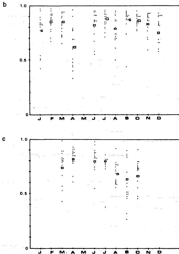
FIGURE 1 (Continued) Variations of the absolute value of the correlation coefficient of K and n versus month for each station. The square means all stations merged together. b) 12–13 h UT; c) 15–16 h UT.
