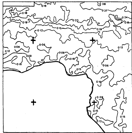
Figure 5. a) Albedo map for week #42 (October) 1984. b) Albedo isolines for week #42.
