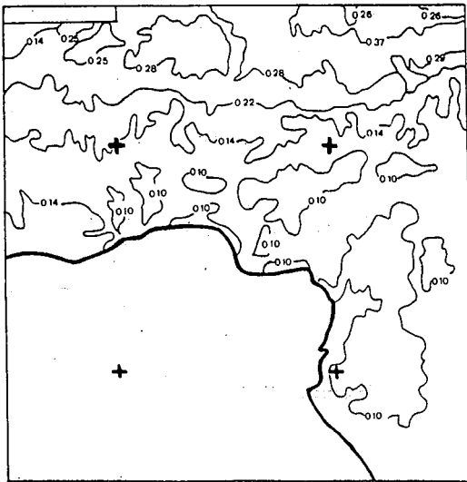
Figure 4. a) Albedo map for week #21 (May) 1984. b) Albedo isolines for week #21.
