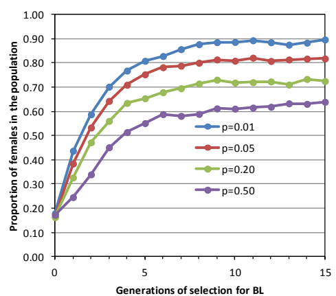
Figure 3-6: Simulated proportion of females over generations of selection for body length for different proportions selected ( p ).
