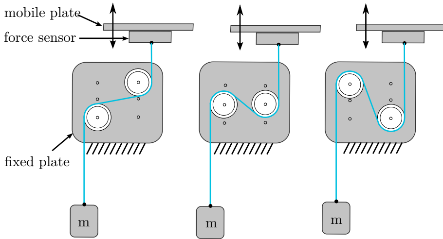
Figure 4.9: Experiment for guiding friction estimation
