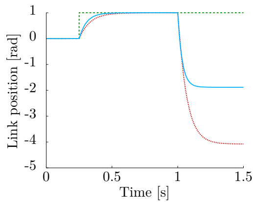
Figure 14.4: Simulation: Comparison between the SDRE controller and the fixed gains controller for a link positioning task. The green/dashed line is the desired link position. The light blue/solid and red/dotted lines depict the link position with the SDRE controller and the fixed gains controller.
