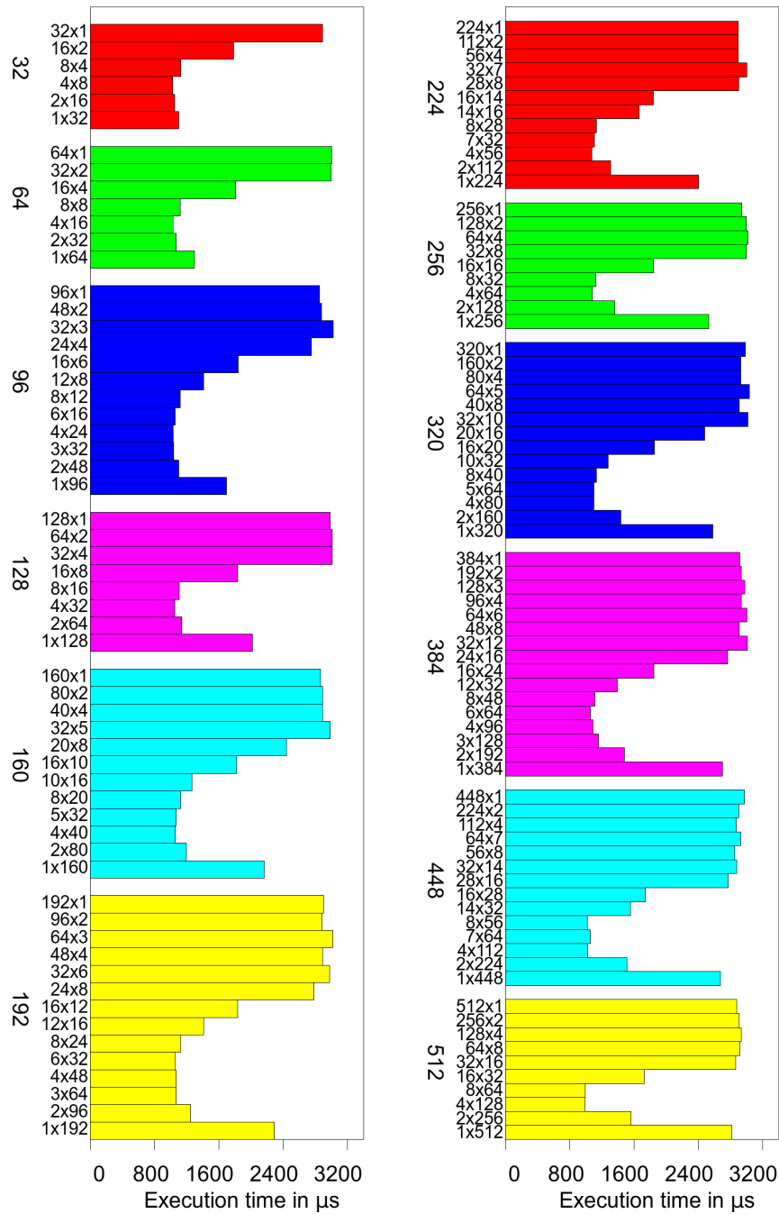
Figure 7.3: Impact of block dimensionality on performance for different block sizes expressed in \mu s for G80 architecture. The reference kernel here is the main loop nest from syrk (Polybench suite) shown in Figure 5.14 page 163.
