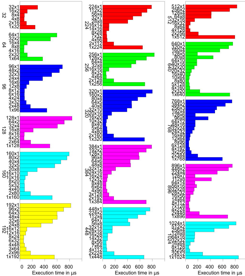
Figure 7.6: Impact of block dimensionality on performance for different block sizes expressed in \mu\text{s} for Kepler architecture. The reference kernel here is the main loop nest from syrc (Polybench suite) shown in Figure 5.14 page 163.
