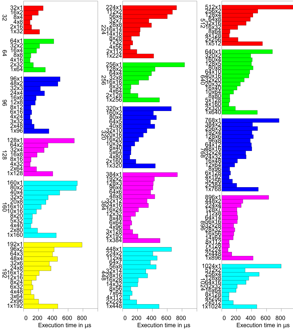
Figure 7.5: Impact of block dimensionality on performance for different block sizes expressed in \mu\text{s} for Fermi architecture. The reference kernel here is the main loop nest from syrc (Polybench suite) shown in Figure 5.14 page 163.
