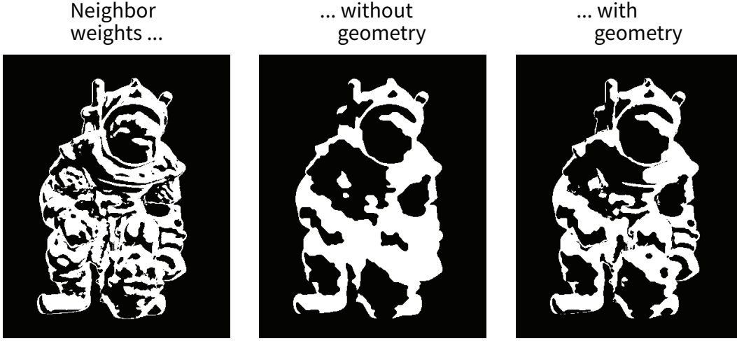
Figure 3.8: The left-most image shows a segmentation with neighbor weights equal to zero which results in mere thresholding. In the middle image the neighbor weights are set to a constant value of \tilde{N} = 0.5 , whereas the right image has the same base \tilde{N} but uses the geometry terms to modulate the neighbor weight.
