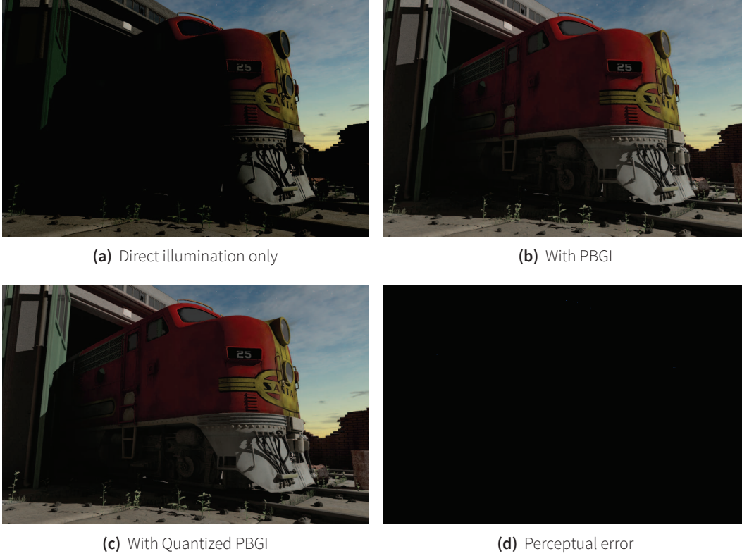
Figure 6.10: A more complex example (LUT with 10 000 clusters).
