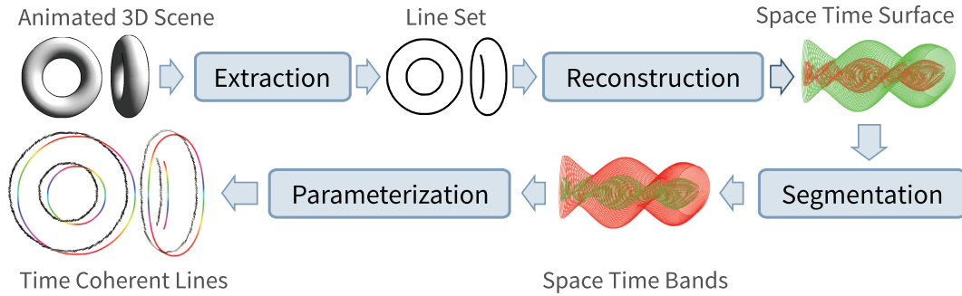
Figure 4.4: Overview: lines are extracted independently for each frame of the animation, before being grouped as plausible corresponding lines from frame to frame. Lines may split or merge during the animation and create a graph which is subsequently decomposed in bands corresponding to single lines over time. These bands, or space-time lines, are finally parameterized independently under user control to provide time-coherent parametric lines.
