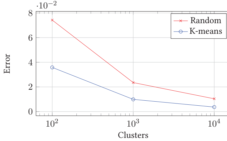
Figure 6.7: Approximation quality for random and k-means cluster LUT in the «Big Buck Bunny» scene. The error is the average of the absolute mean error between each node's actual data and its approximation.
