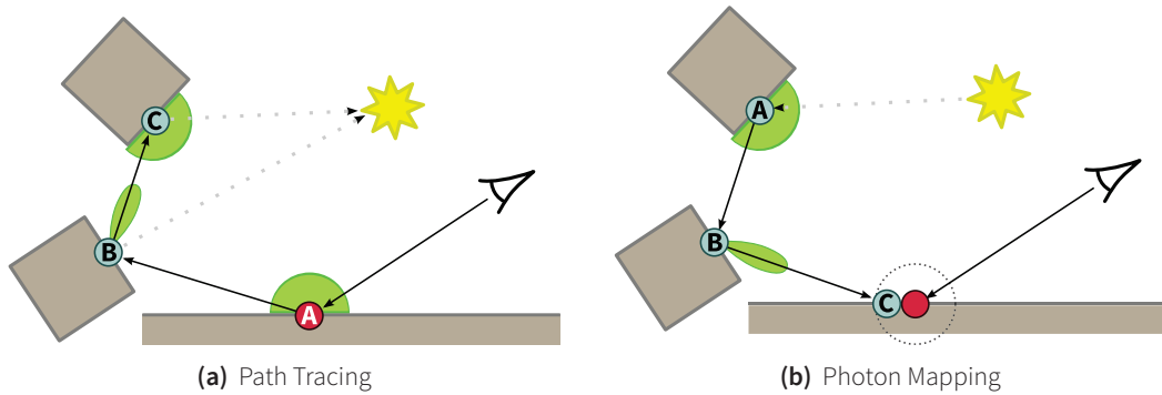
Figure 5.4: Path Tracing: Path tracing starts from the eye and constructs paths through the scene. From the primary hit point A, a secondary ray is generated by sampling the BRDF at this point. This ray hits B, lying on a glossy surface. From there, another element for the path is generated hitting C and so on. At each hit point, connections are also made to all light sources. Photon Mapping: Photons are emitted from the light sources. Here, a photon hits a diffuse surface in point A and is recorded in the photon map and is then, by sampling the BRDF in A, bounced in the direction of B. There it is recorded again and bounced off again, finally recorded in C. To calculate the indirect light at the visible points (as an example the red point), the photon map is queried for all recorded points in a certain radius around the point. The final indirect light value is computed as the weighted sum of the returned points.
