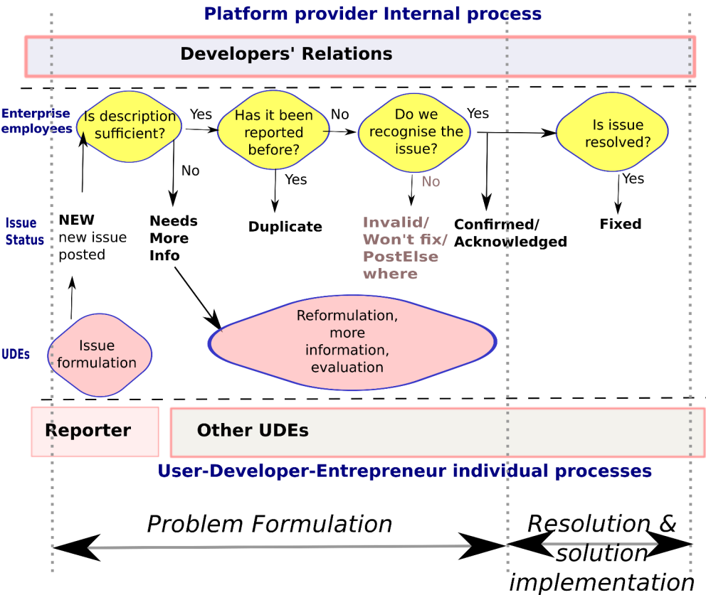
Figure 17.11: The conversational process followed in the developer support forum during an issue resolution. Status indications are providing a level of transparency regarding internal platform resolution process, while the debate among the community aims to clarify and evaluate the issue under review.
