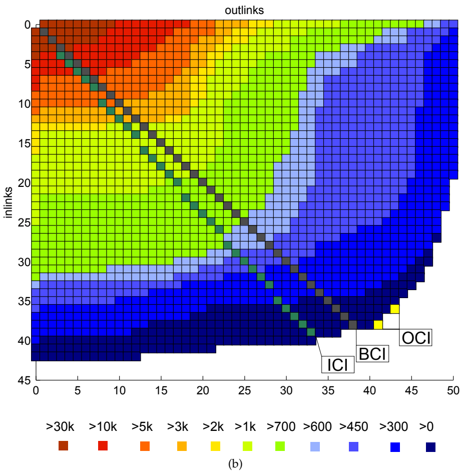
Figure 2.3: a. The differentials \partial^{\text{out}}\Lambda_D and \partial^{\text{in}}\Lambda_D for the digraph formed by Wikipedia. White squares indicate a value of zero. b. The D-core matrix of the Wikipedia 2004 digraph
