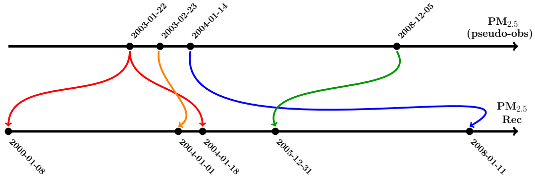
Figure 4.4: Re-sampling PM_{2.5} pseudo-observations over the learning period. The analog day of 31 December 2005 is 5 December 2008 (green arrow), the analog day of both 18 January 2004 and 8 January 2000 is 22 January 2003 (red arrow).
