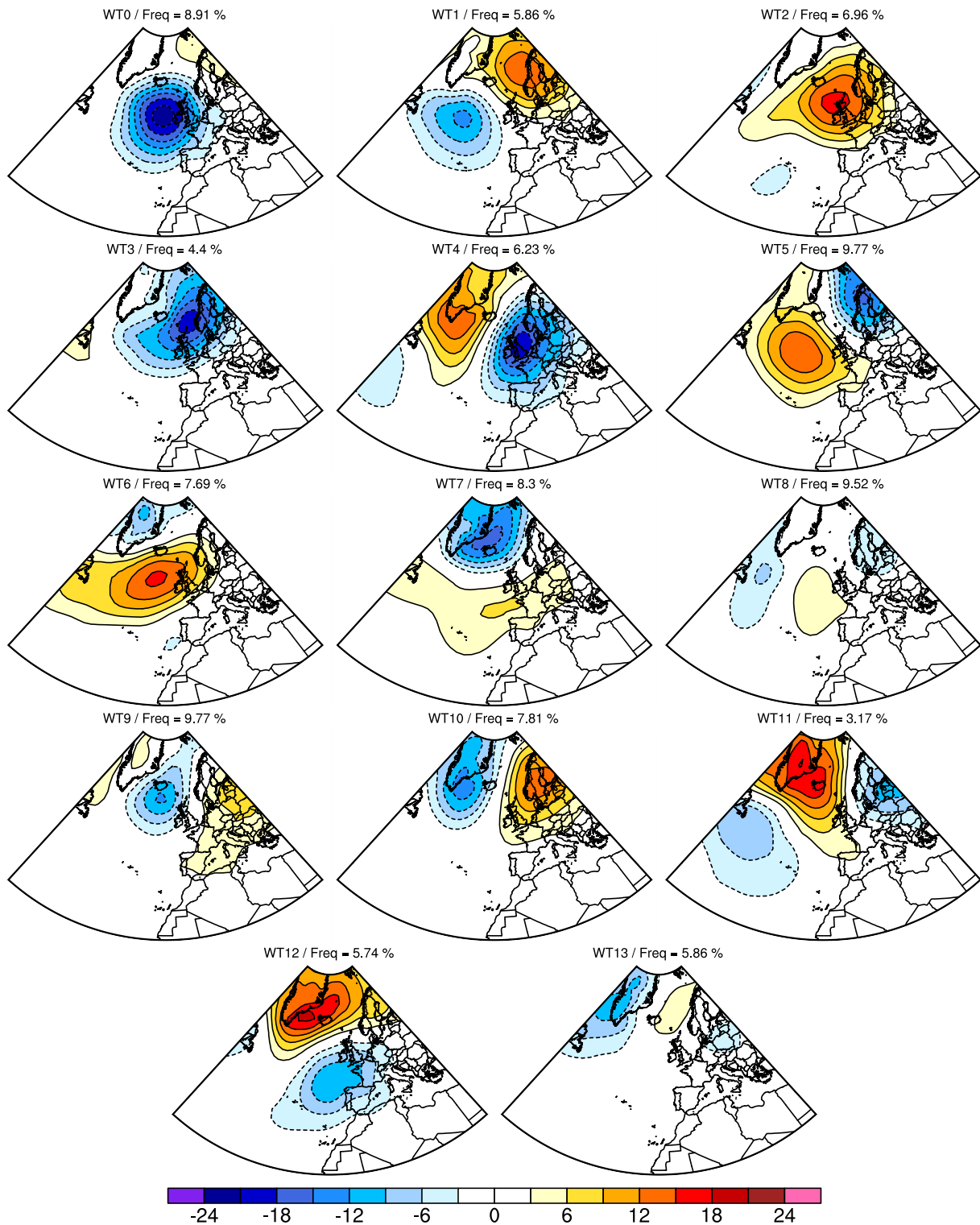
Figure B23: PSL anomalies (expressed in hPa) of the 14 WTs in SON, built on the learning period (2000-2008). The frequency of each WT is stated above the corresponding WT.
