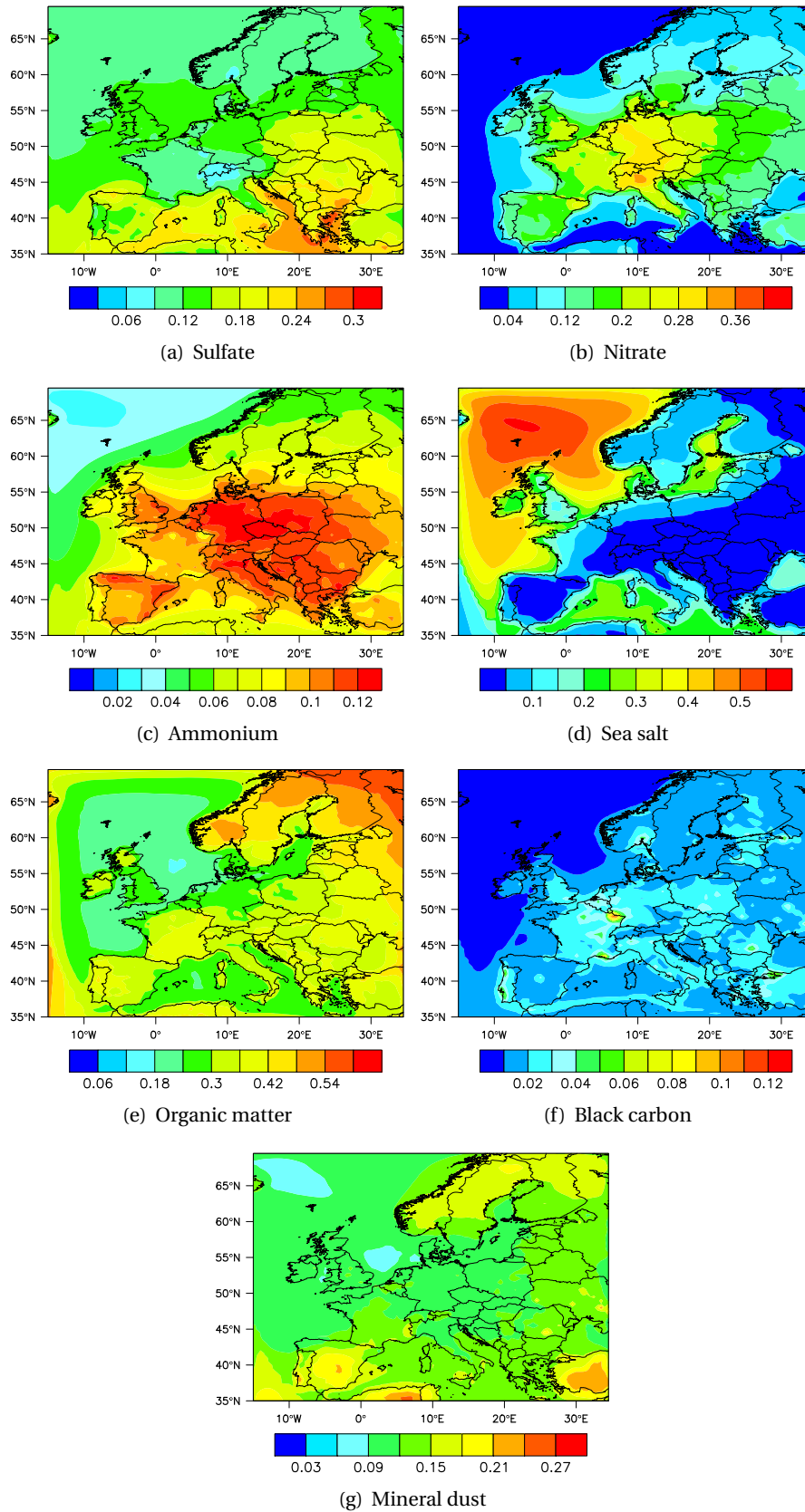
Figure 3.3: Nine-year (2000-2008) averaged surface fractions of sulfate, nitrate, ammonium, sea salt, organic matter, black carbon and mineral dust in PM_{2.5} .
