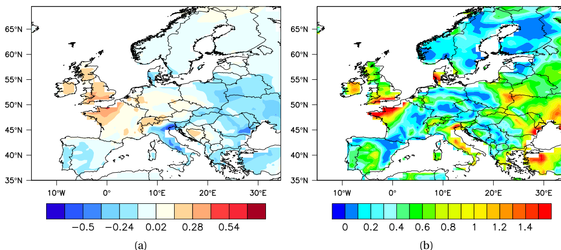
Figure 4.10: (4.10a) Difference between the annual PM_{2.5} concentration ( \mu\text{g m}^{-3} ) in the near future and in the historical period; (4.10b) ratio of PM_{2.5} changes due to climate change and PM_{2.5} interannual variability under the RCP4.5 scenario.
