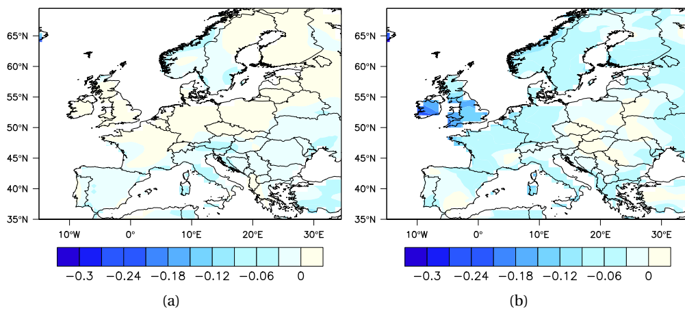
Figure B19: Difference between the annual wind speed ( \text{m s}^{-1} ) in the distant and near future for the RCP4.5 (a) and RCP8.5 (b) scenarios.
