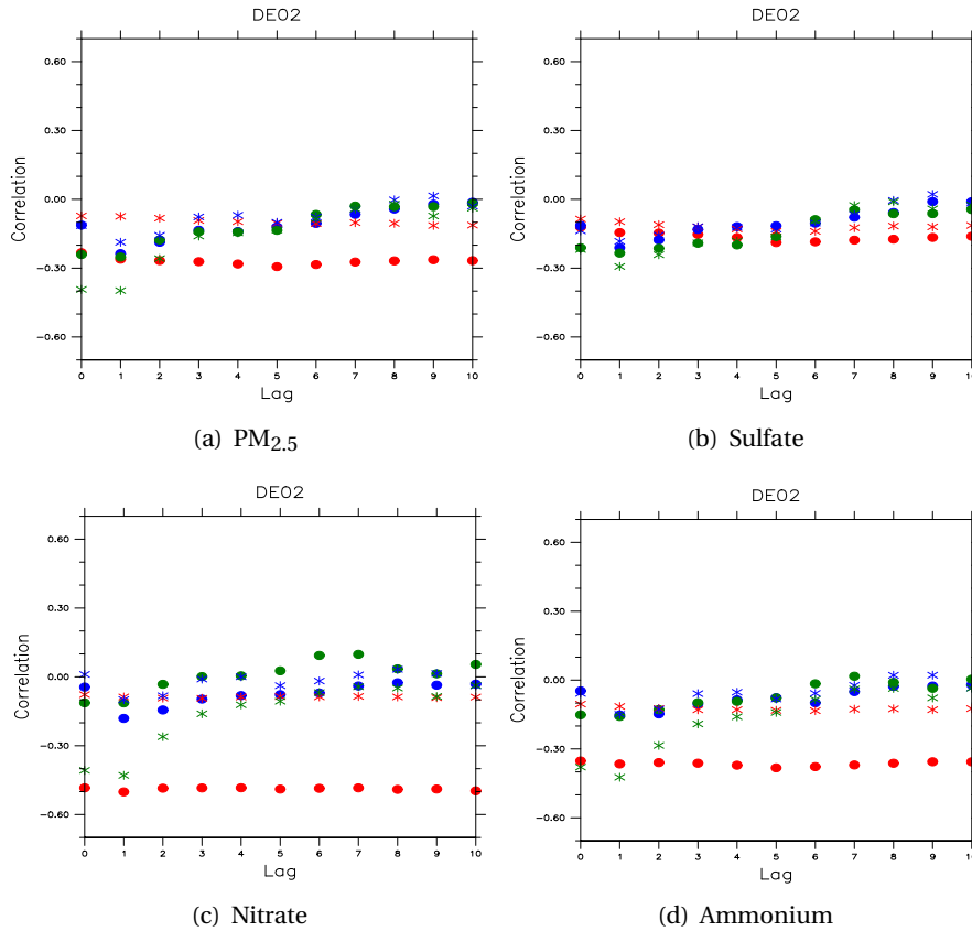
Figure 3.5: Correlations between meteorology (temperature in red, precipitation in blue, wind speed in green) on a given day and pollutant concentrations ( PM_{2.5} , sulfate, nitrate and ammonium), ranging up to 10 days after at DE02 (2006-2008). Simulated data are represented with a star, while observational data are represented with a dot.
