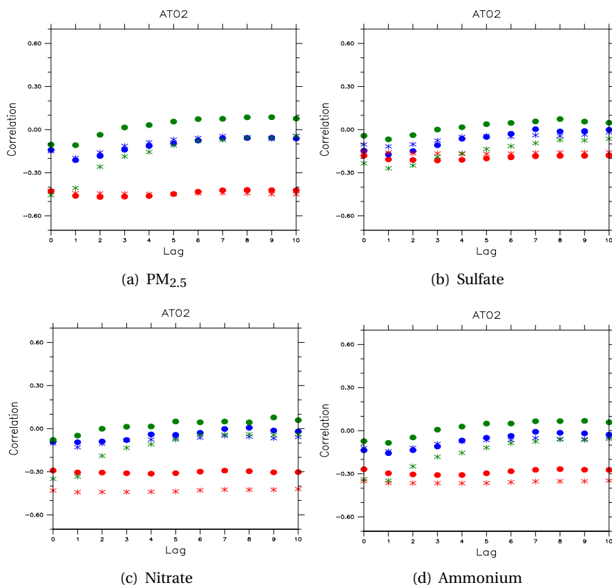
Figure 3.4: Correlations between meteorology (temperature in red, precipitation in blue, wind speed in green) on a given day and pollutant concentrations (PM 2.5 , sulfate, nitrate and ammonium), ranging up to 10 days after at AT02 (2003-2008). Simulated data are represented with a star, while observational data are represented with a dot.
