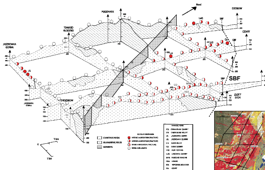
Figure 61 – 3D block showing the extent of the reddening/albitization alterations in the Kłodzko Złoty-Stok Massif (KZS). The albitized granitoïd domain appears as contiguous to the non-albitized granitoïd domain. The limit between the reddened/albitized and the light/unstained granitoïdes coincides with a fault plane (underlined in grey) parallel to that proposed by Cymerman (2004). The 3D block was obtained by assembling the serial 2D sections along the traces shown on the inset geological map. SBF = Sudetic Boundary Fault.
