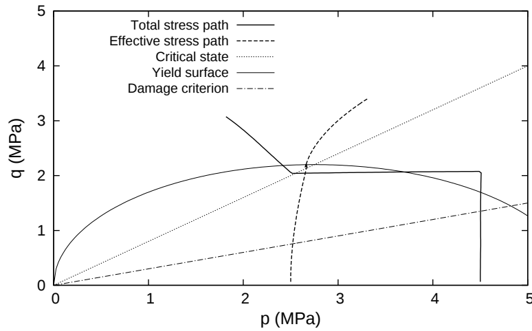
Fig. 7.26: Total and effective stress paths at the tunnel wall
