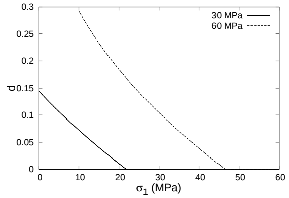
Fig. 6.16: Damage evolution as a function of radial stress
