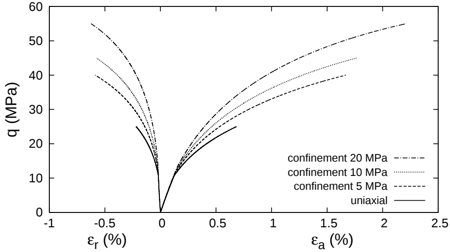
Fig. 6.9: Stress-strain curves for different confining pressures
