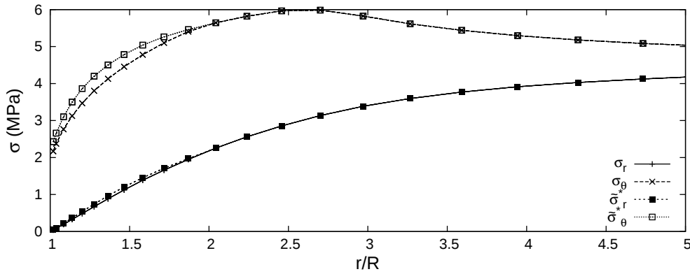
Fig. 7.17: Total and double effective stress for saturated state
