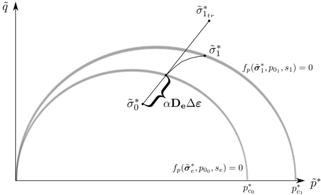
Fig. 5.5: Explicit algorithm for plasticity
