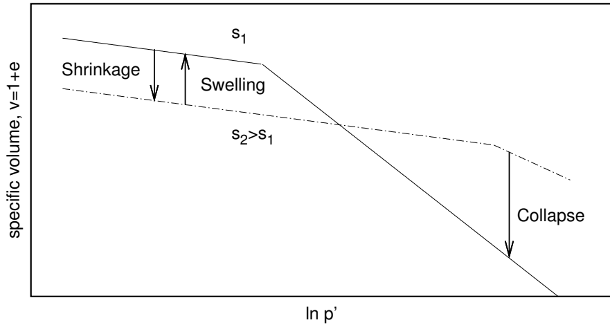
Fig. 1.4: Influence of suction on volumetric compression and volume changes due to wetting and drying
