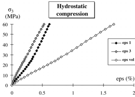
Fig. 6.2: Hydrostatic compression test (Shao et al., 2006)
