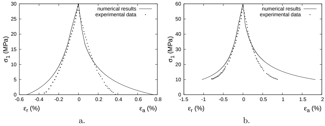
Fig. 6.14: Lateral extension tests (a. p_c = 30 MPa, b. p_c = 60 MPa)
