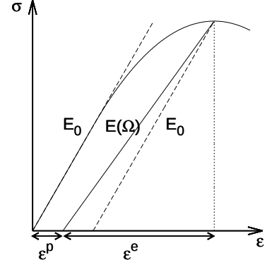
Fig. 3.3: Coupling of damage and plasticity
