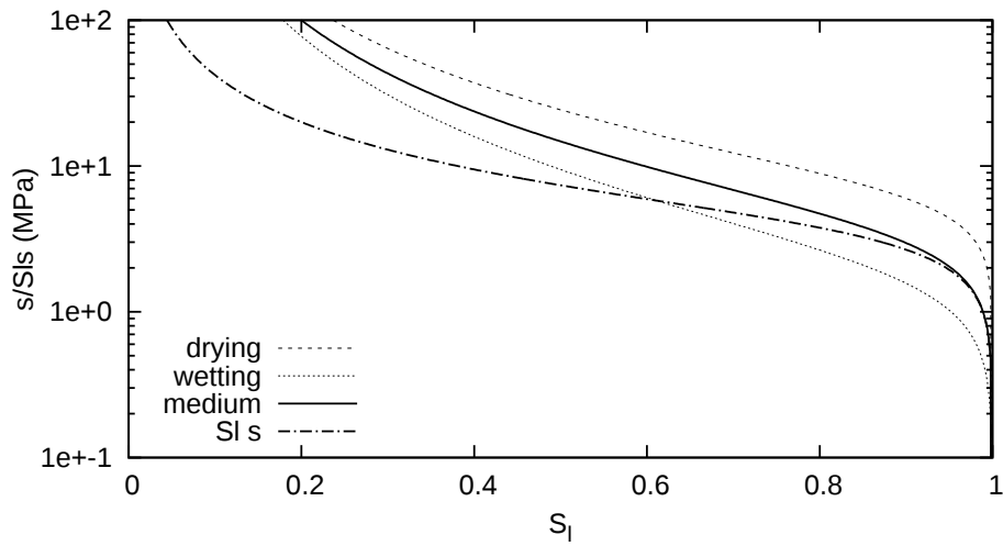
Fig. 6.21: Water retention curve and S_l s component of effective stress for Boom clay
