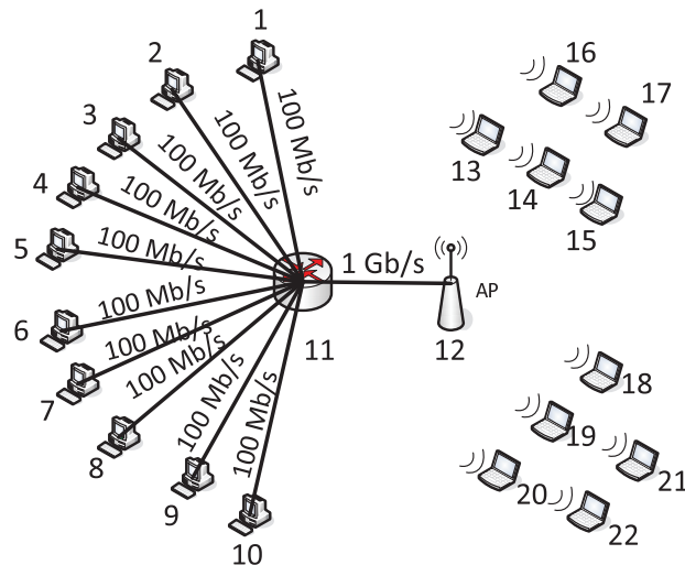
Figure 7.1: Network topology
