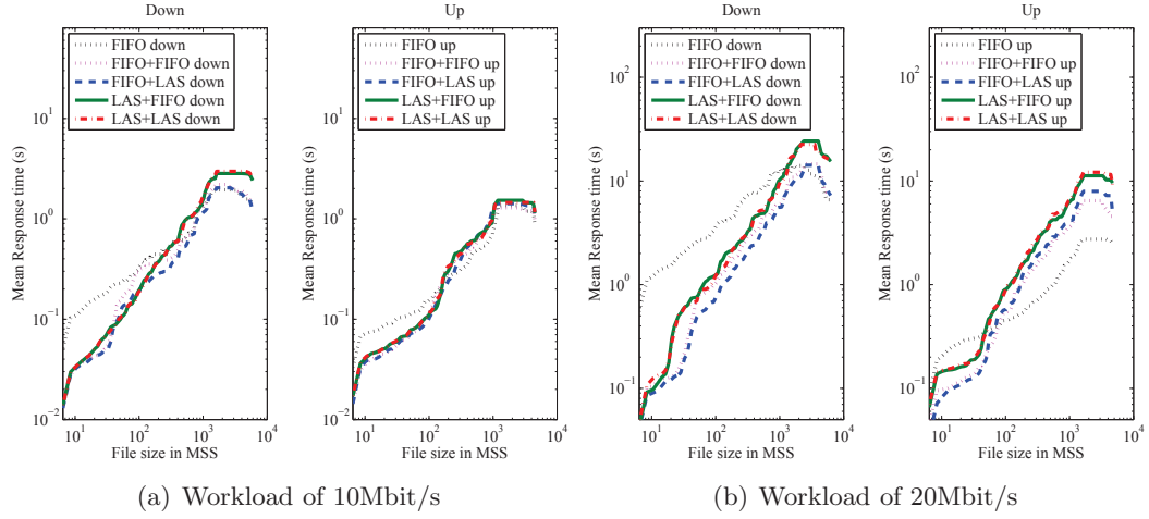
Figure 3: Comparison between various queueing policies in EFD queues – Average response time, symmetric load, packet-based
