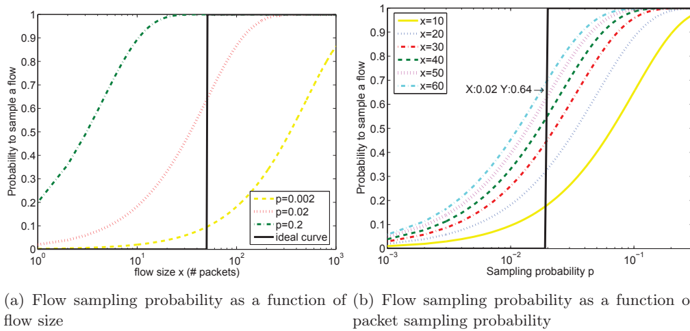
Figure 3.1: Flow sampling probability P_s , in which T_s=1
