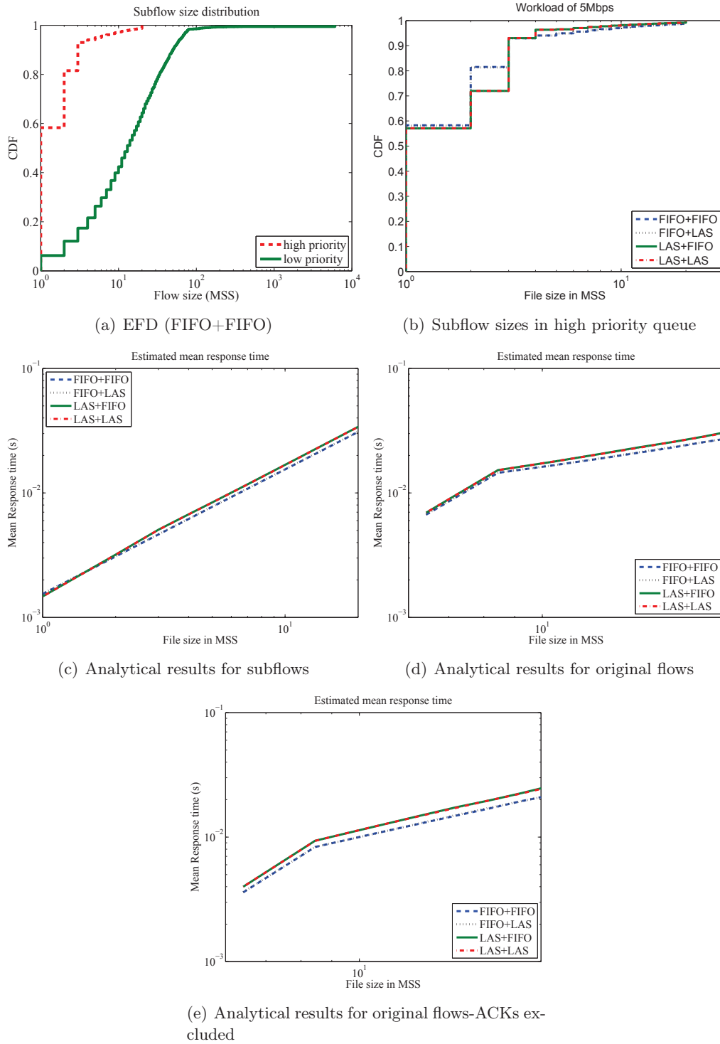
Figure 5.17: An Alternative for Modeling EFD's variants
