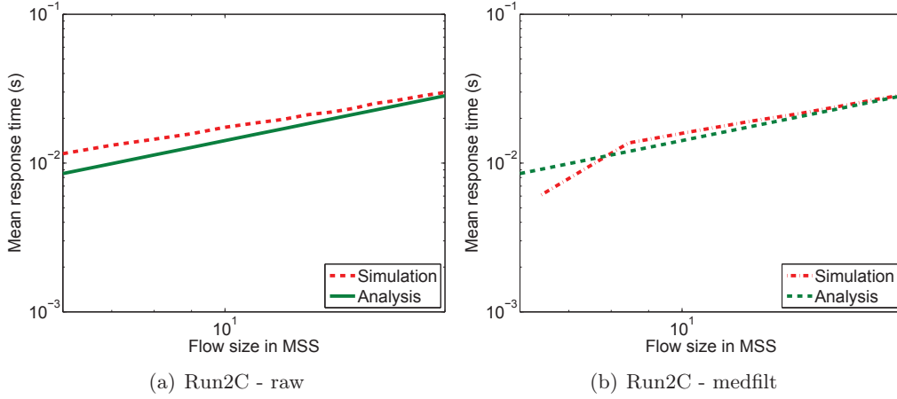
Figure 5.6: Analysis and Simulation, \rho = 0.5 , Run2C
