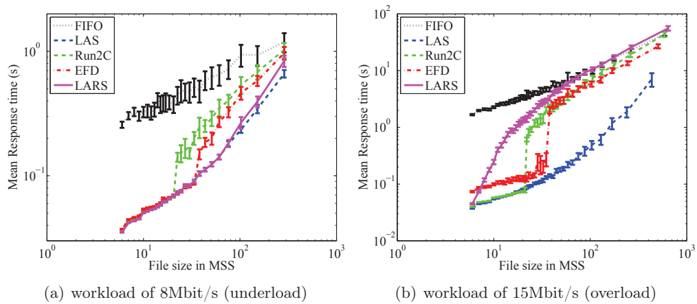
Figure 4.10: Confidence interval of response time over flow size
