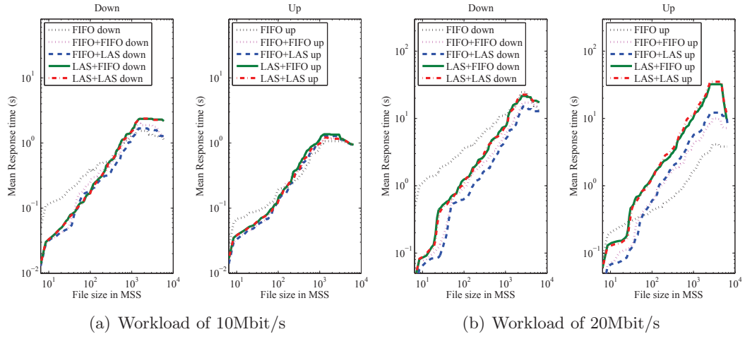
Figure 2: Comparison between various queueing policies in EFD queues – Average response time, symmetric load, byte-based
