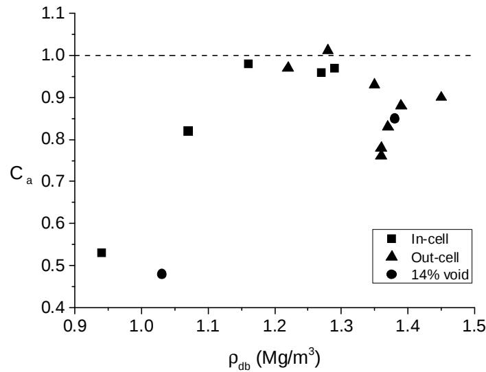
Figure 7. Anisotropy coefficient changes with respect to bentonite dry density for different test conditions. From Fig. 3, the most marked peaks in the swelling pressure evolution are observed in the tests with medium range of bentonite dry densities. As explained previously, peaks indicate a collapse in the microstructure that favours the development of an isotropic microstructure. This explains the isotropic behaviour shown in Fig. 7 for the samples with medium bentonite dry densities and an anisotropy coefficient close to 1.
