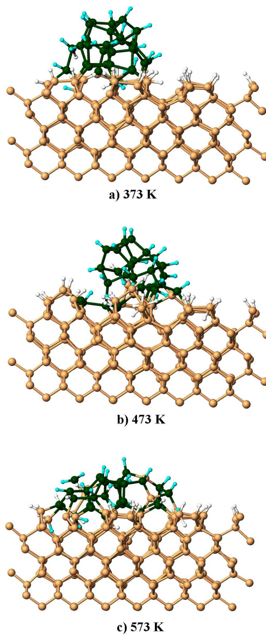
FIGURE 5.21: Snapshots of the atomic configurations at 200 ps after the impact of the \text{Si}_{29}\text{H}_{24} cluster with the surface for various substrate temperatures: a) 373, b) 473, and c) 573 K. The impact energy is always 2.74 eV/atom.
