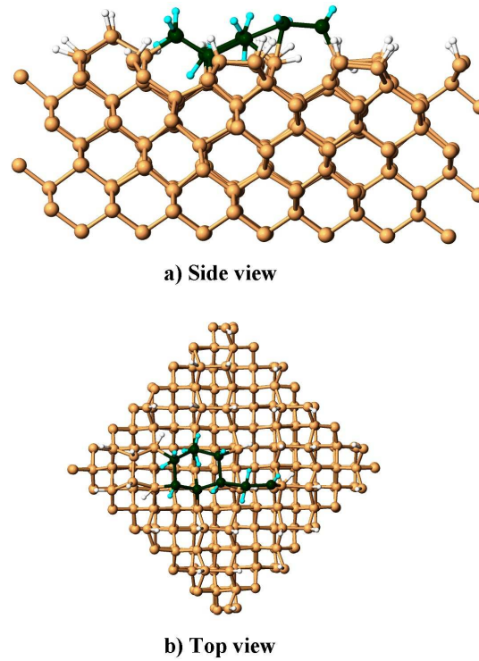
FIGURE 5.11: Side and top view of the atomic configuration after the cooling down to 573 K for the case of the \text{Si}_8\text{H}_{12} cluster approaching the substrate with an impact energy of 5.23 eV/atom.
