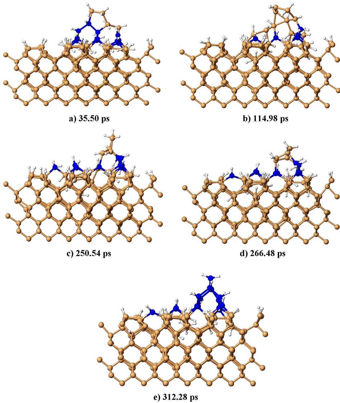
FIGURE 4.8: The structure evolution of the silicon surface after the 12 H-atom exposure, at a surface temperature around 1616 K. The blue atoms represent the silicon atoms found in epitaxial positions.
