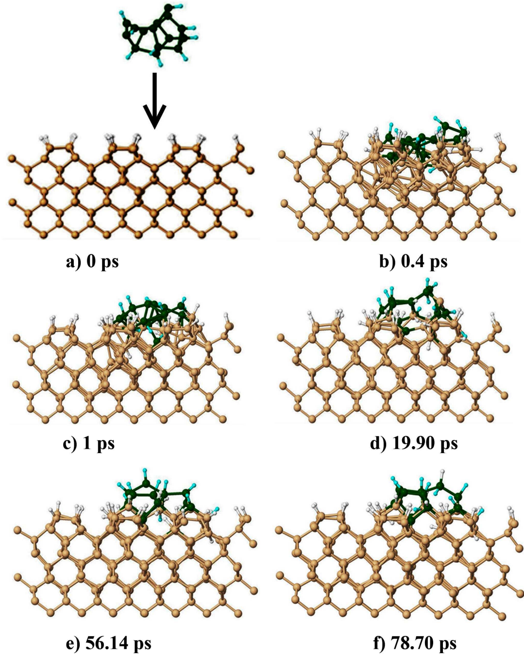
FIGURE 5.2: Snapshots of atomic configurations at various times during the \text{Si}_{15}\text{H}_{10} cluster surface collision with an impact energy of 5.3 eV/atom and a substrate temperature of 373 K. The large brown spheres represent the surface silicon atoms while the green ones represent silicon atoms of the \text{Si}_{15}\text{H}_{10} cluster. The small white spheres represent surface hydrogen atoms while the cyan ones represent hydrogen atoms of the \text{Si}_{15}\text{H}_{10} cluster. The same colors will be used to display atomic configurations of the following investigated trajectories.
