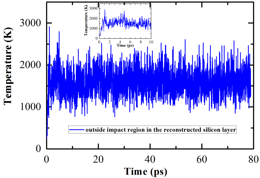
FIGURE 5.4: Time evolution of the instantaneous temperature of substrate atoms surrounding the impact region in the reconstructed silicon layer after the \text{Si}_{15}\text{H}_{10} cluster-surface impact. The insert indicates a rapid increase of the temperature of those atoms from 373 K to about 3000 K and a subsequent decrease to an equilibrated temperature of 1600 K.
