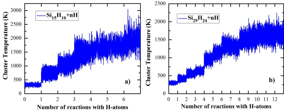
FIGURE 3.2: The evolution of the instantaneous temperature of clusters with the number n of reactions with H-atoms: a) \text{Si}_{15}\text{H}_{10} ; b) \text{Si}_{29}\text{H}_{24} .
