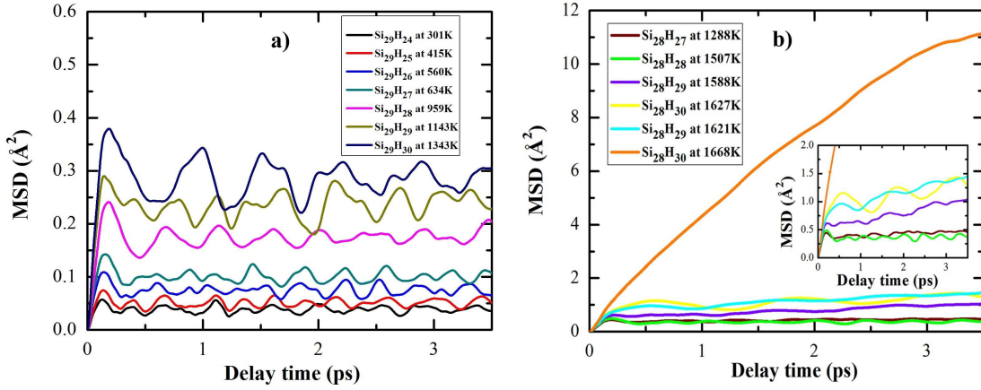
FIGURE 3.5: MSD of silicon atoms of the \text{Si}_{29}\text{H}_{24} cluster at different temperatures due to the subsequent reactions with H-atoms: a) first six reactions with H-atoms; b) last six reactions with H-atoms.
