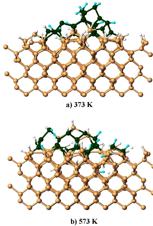
FIGURE 5.19: Snapshots of the atomic configurations at 200 ps after the impact of the \text{Si}_{28}\text{H}_{13} cluster with the surface for different substrate temperatures: a) 373 K; b) 573 K. The impact energy is always 2.84 eV/atom.
