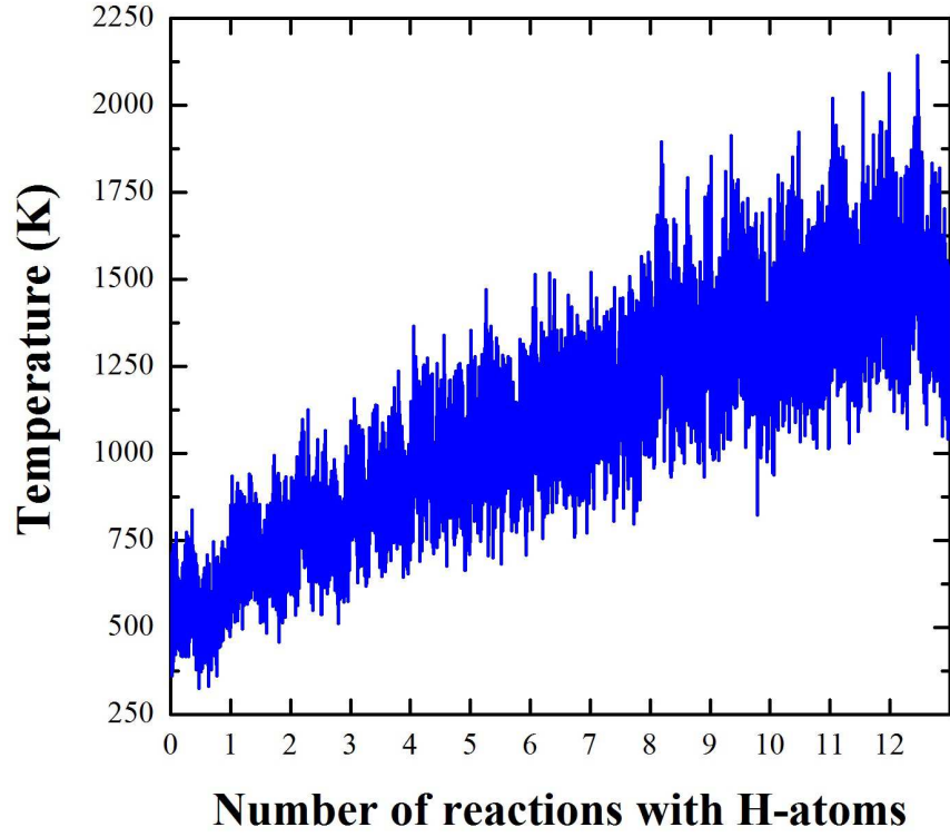
FIGURE 4.6: The evolution of the instantaneous temperature of the cluster atoms together with the substrate atoms touching the cluster as function of the number of reactions with H-atoms.
