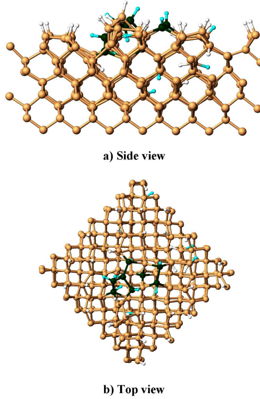
FIGURE 5.17: Side and top view of the atomic configuration at 200 ps after the collision for the case of the \text{Si}_8\text{H}_{12} cluster approaching the substrate at 573 K with an impact energy of 9.95 eV/atom.
