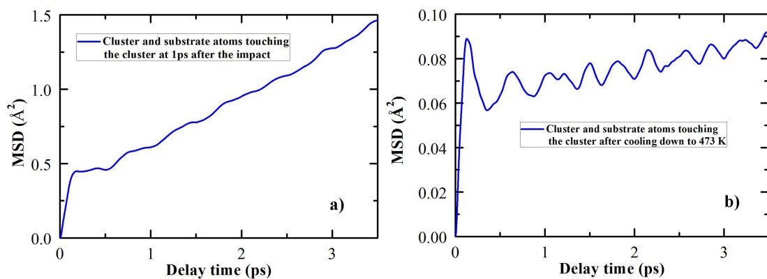
FIGURE 5.16: MSDs of silicon atoms of the \text{Si}_8\text{H}_{12} cluster and substrate silicon atoms touching the cluster for the case of the \text{Si}_8\text{H}_{12} cluster approaching the substrate at 473 K with an impact energy of 9.95 eV/atom: a) at 1 ps after the impact; b) after the cooling down to 473 K.
