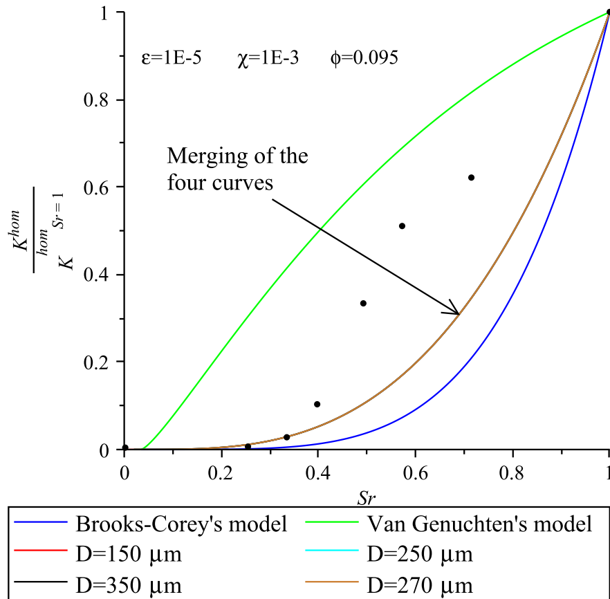
Figure 6.7: The evolution of the relative permeability coefficient K^{hom} / K_{Sr=1}^{hom} with saturation degree Sr for Fontainebleau sandstone (red curves); the fitting parameters of Brooks-Corey's model and Van Genuchten's model are given in [65]; the black circle points are from experiments in [65].
