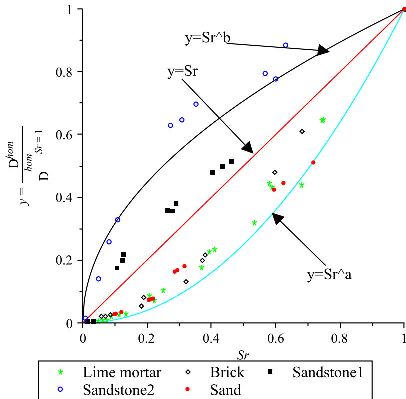
Figure 4.1: Evolutions of the normalized diffusion with saturation degree for several porous materials, D^{hom}_{Sr=1} is the effective diffusion coefficient in saturated porous media, while D^{hom} is the diffusion coefficient in unsaturated case, Sr is the saturation degree, a and b are the exponent coefficients, experimental results are after [6, 33, 159].
