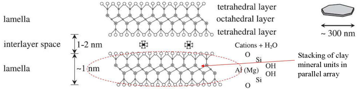
Figure 2.7: Schematic representation of particles which are composed of lamellas and interlayer space[150].
