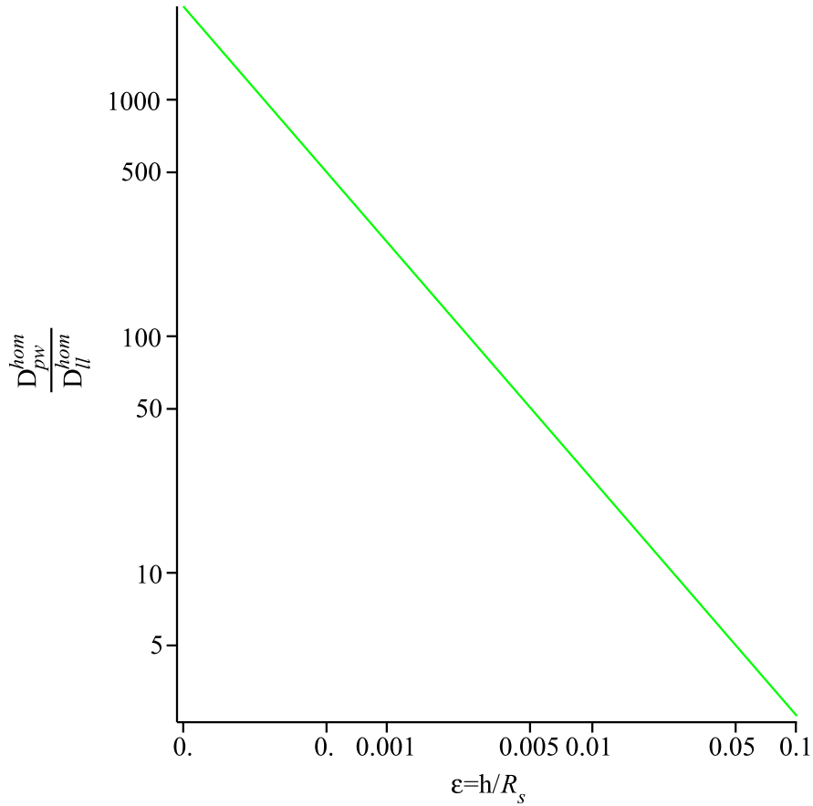
Figure 4.12: Dependence of \frac{D_{pw}^{hom}}{D_{ll}^{hom}} on \epsilon , \phi = 0.4 , the constrictive factor \delta = 0.5 .
