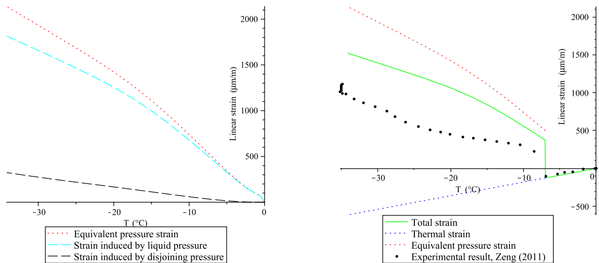
(a) Strains induced by each component of equivalent pressure
