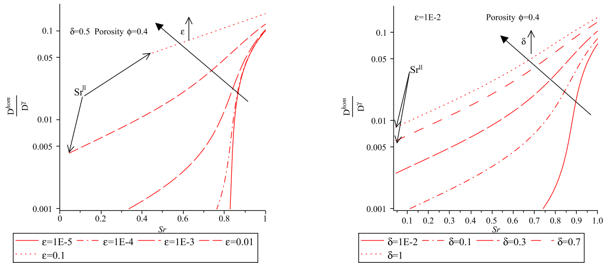
(a) The effect of \epsilon on homogenized diffusion coefficient D^{hom} .
