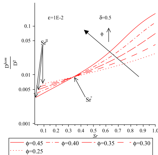
(c) The effect of \phi on homogenized diffusion coefficient D^{hom} .
