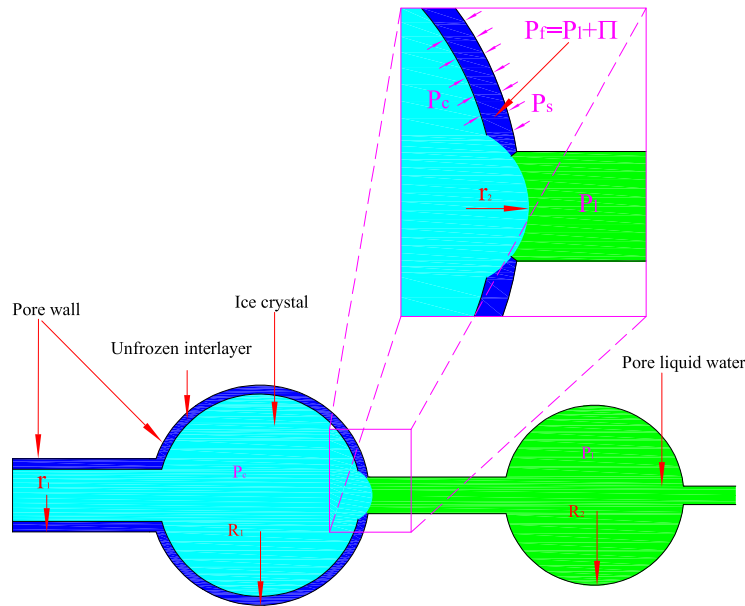
Figure 7.6: Schematic illustration of disjoining pressure of water film within crystallized pores.
