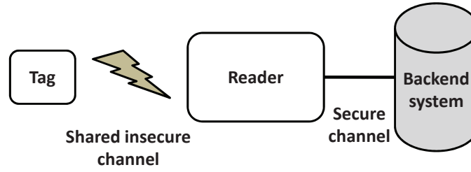
Figure 3.1: RFID environment
