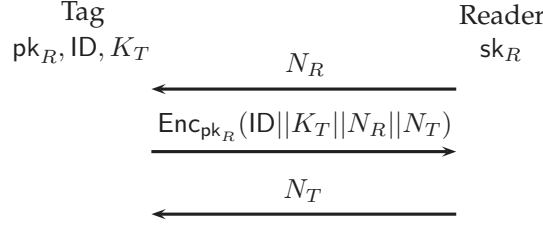
Figure 3.10: RFID authentication protocol based on public key cryptography
