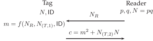
Figure 3.9: RFID authentication protocol based on Rabin cryptosystem
