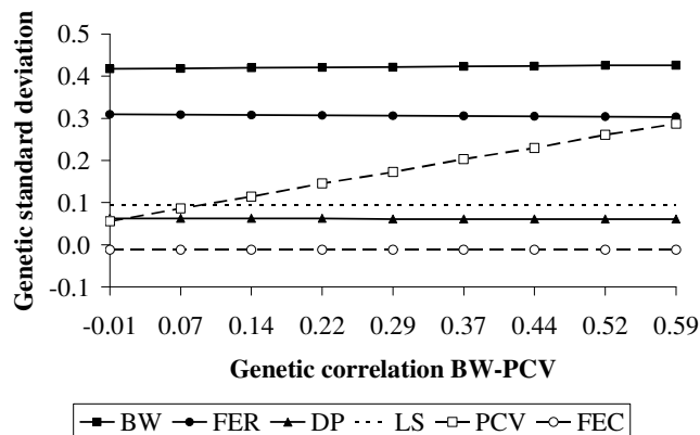
Figure 5. Expected selection responses in genetic SD according to the genetic correlation between BW and PCV in the Hcombined breeding goal. H_{combined} = 7.69 \times A_{BW} + 1.38 \times A_{FER} + 3.53 \times A_{DP} + 3 \times 10^{-4} \times A_{PCV} - 18.85 \times A_{FEC} where A is the true breeding value, FER = Fertility, DP = dressing percentage, LS = litter size, PCV = packed cell volume, FEC = fecal egg count.
