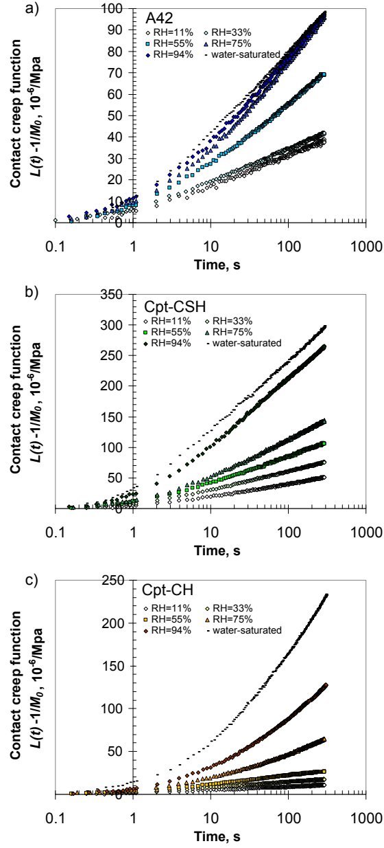
Figure 8.2: Median contact creep function of a) C 3 S paste, b) compact of C-S-H and c) compact of CH, at various relative humidities. For C 3 S paste in water-saturated conditions, we take C 3 S paste tested at age of 56 days in water-saturated conditions from section 6.3. For compacts, the results in water-saturated conditions are from section 7.3.
