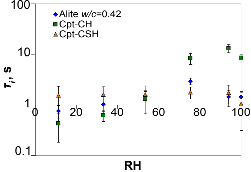
Figure 8.5: Indentation characteristic time \tau_i of C_3S paste, compact of C-S-H and compact of CH in equilibrium with various relative humidities.
