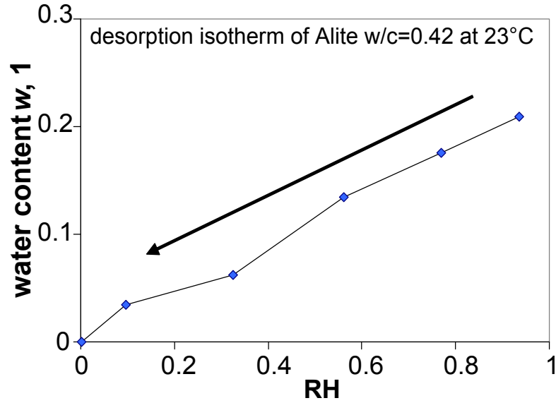
Figure 8.6: Desorption isotherm of a 180-days-old \text{C}_3\text{S} paste cured in water, with water-to-cement ratio w/c=0.42 .
