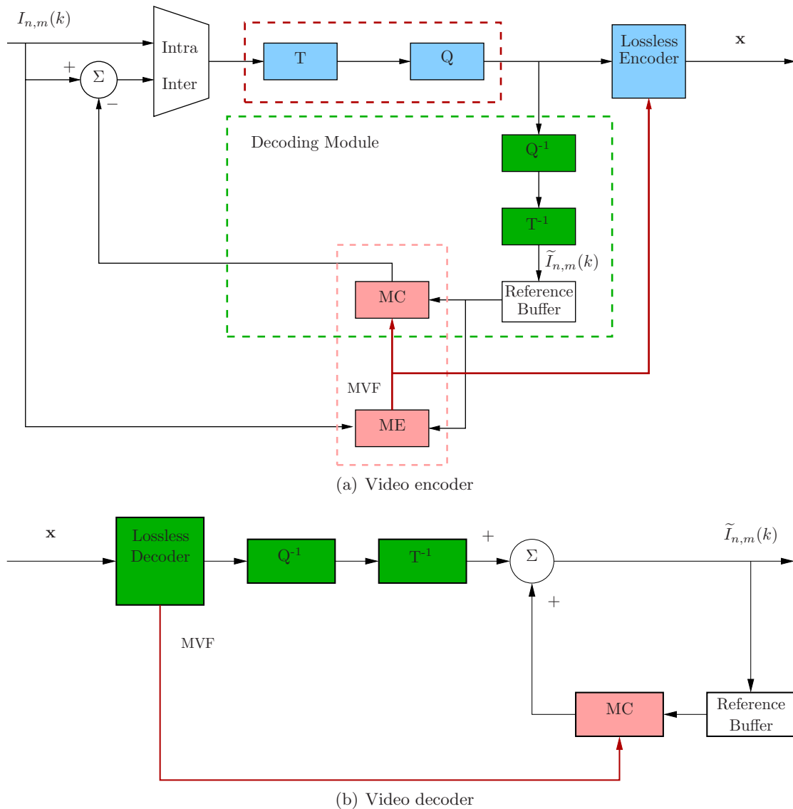
Figure 1.3: Structure of a video codec.
