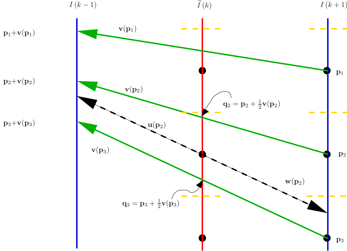
Figure 2.7: Bidirectional motion estimation in DISCOVER. Green solid arrows: results of forward ME. Black dashed arrows: results of bidirectional ME for the block centred in \mathbf{p}_2 .
