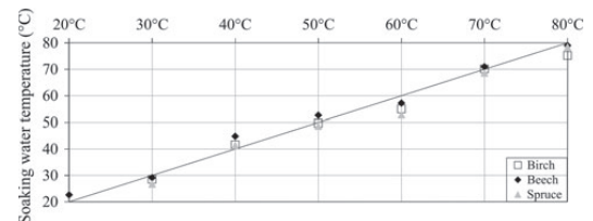
Fig. 1 Effective soaking water temperature as compared to target temperature
