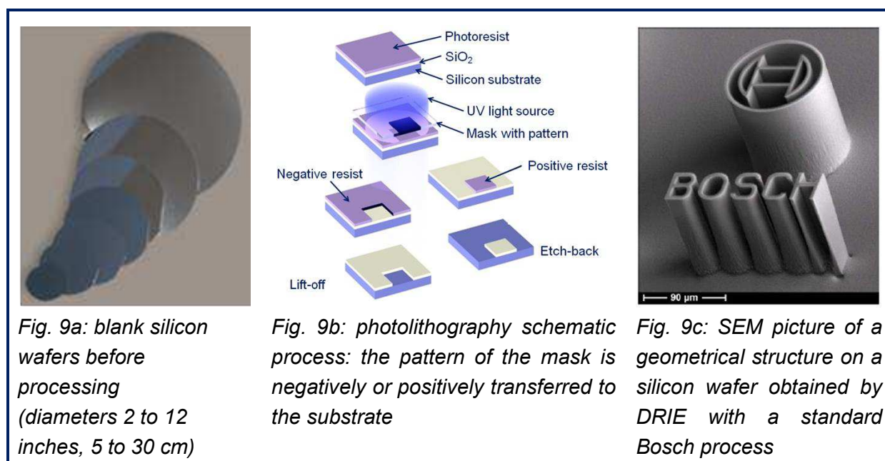
Fig. 9: substrate micro machining processes
