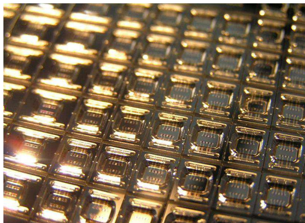
Figure 10b: batch fabrication of micro thermal conductivity detectors; unit size is 7 \times 5 \text{ mm}^2 ; 100 units are fabricated on one wafer.
