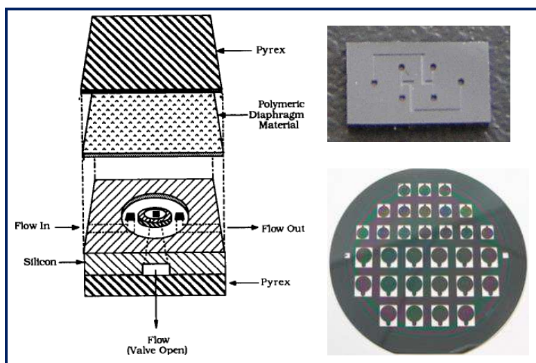
Fig. 32a: examples of micro injectors: left: pneumatic injector by Bruns [74] top right: pneumatic injector developed at MEMS TC by Nachev [75,76] ; chip size 4 \times 7 \times 1 \text{ mm}^3 bottom right: wafer with two-parts mechanical injectors developed at MEMS TC
