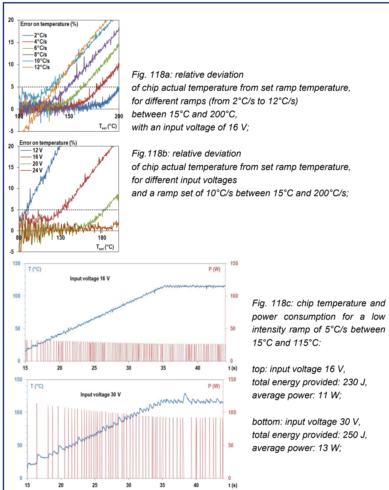
Fig. 118: illustration of the influence of input voltage choice for chip heating; T_{amb}=30^{\circ}\text{C} .
