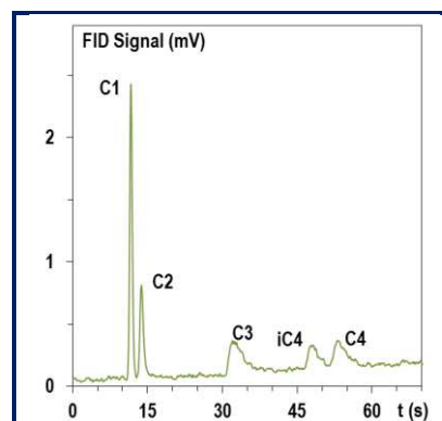
GeoService1, semi-packed column (1.1 m x 200 \mu\text{m} x 100 \mu\text{m} , e_f=1 \mu\text{m} ), P=6.8 bar, V_{inj}=2 \mu\text{L} , T=10^\circ\text{C}-120^\circ\text{C} at 6^\circ\text{C/s} .
