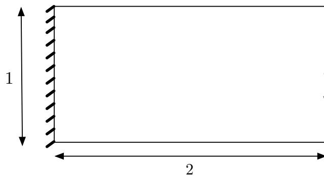
Figure 2.13: Boundary conditions for the 2 \times 1 cantilever.
