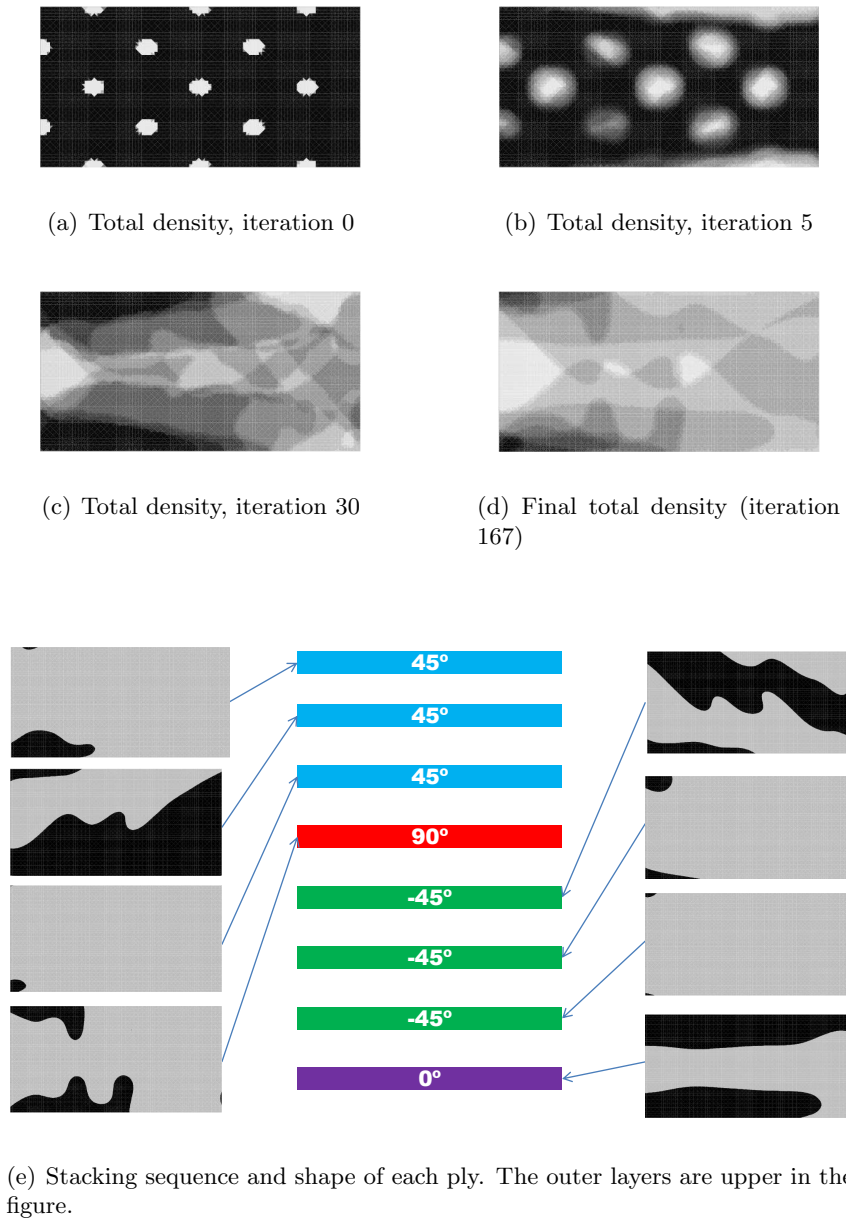
Figure 3.12: Results of Problem 3.9.5 under the second load case (uniform vertical force). (a),(b),(c),(d): Evolution of the total addition of densities of each ply (darker gray means more plies superposed). (e): Optimal stacking sequence and in-plane shape of each ply (black represents material). Sub-figure (d) looks thicker than the superposition of plies in (e) due to the regularization between the the densities and the level-sets.
