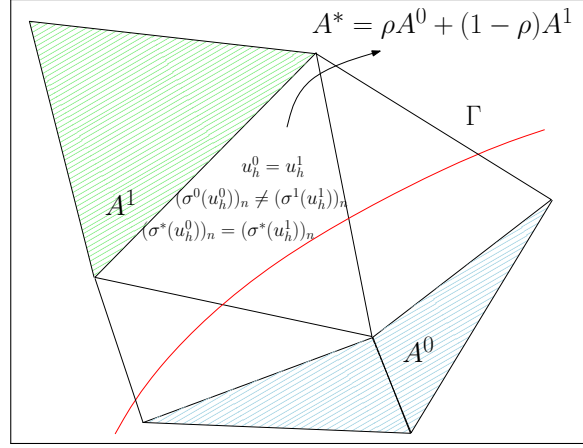
Figure 2.2: Transmission condition in a fixed mesh framework.
