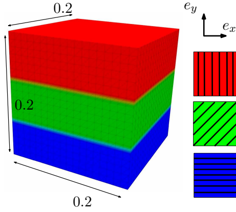
Figure 4.21: Layered cube, and fiber orientation.
