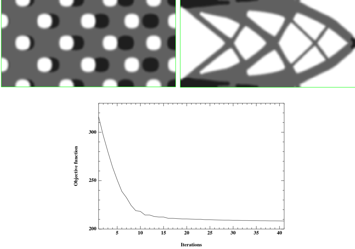
Figure 2.26: Initialization with two materials (top left), optimal shape (top right) and convergence history of the objective function (bottom).
