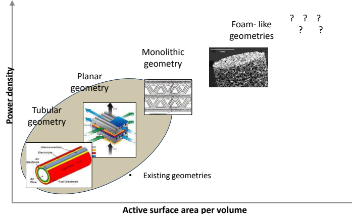
Figure 5.4: Evolution of power density vs active surface of SOFC
