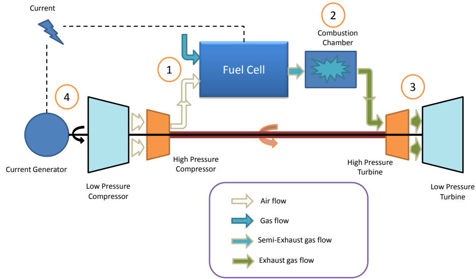
Figure 5.3: Example of an hybrid system.
