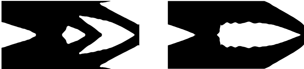
Figure 2.11: Optimal shapes for the using the discrete shape gradient (left) and the continuous formula (right).
