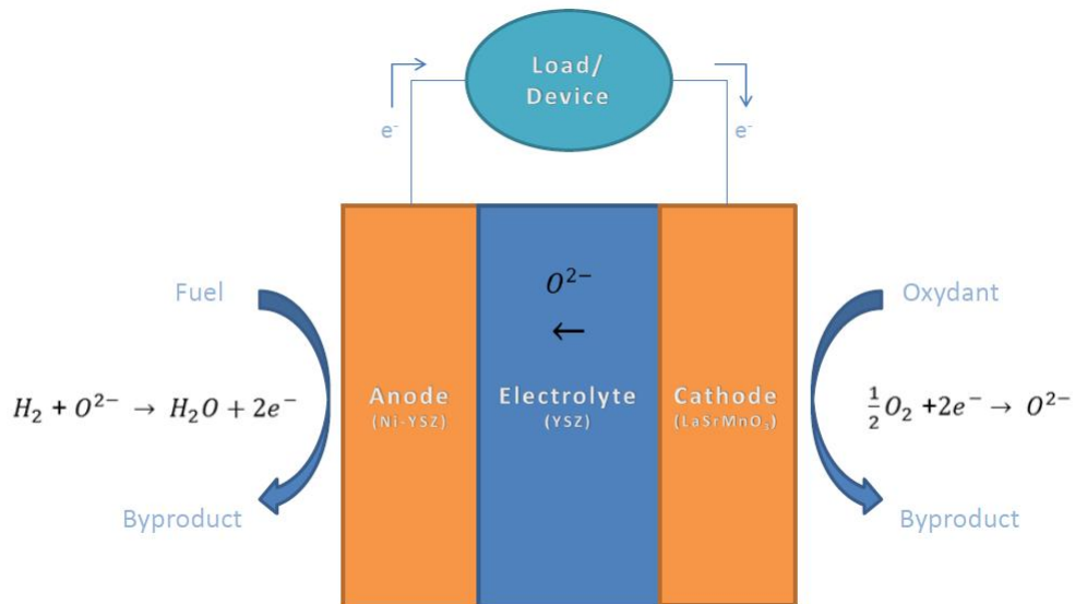
Figure 5.2: Triple structure of a solid oxide fuel cell. The O_2 from the air is consumed in the cathode, meanwhile the O^{2-} ions liberated from the reduction reaction travel through the electrolyte to the anode, where the oxidation reaction of the fuel ( H_2 ) takes place, liberating heat, water and electricity.
