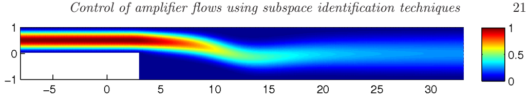
FIGURE 18. Base flow over a backward-facing step at Re = 350 . Colors correspond to the kinetic energy levels.
