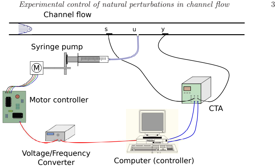
FIGURE 2. Sketch of the full experimental set-up including the air tunnel, all actuation and measurement devices, and data acquisition and processing units.
