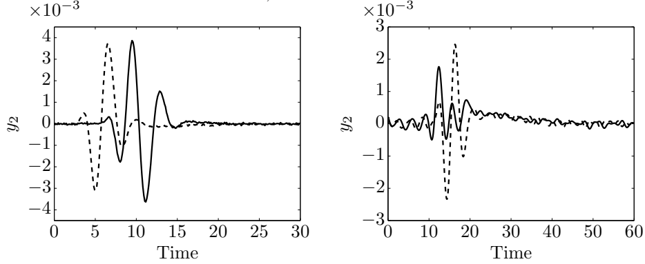
FIGURE 8. Identified impulse response functions: (a) response measured at y_2 for an impulse generated in u_1 (continuous line) and u_2 (dashed line); (b) response measured at y_2 for an impulse in s_1 (continuous line) and s_2 (dashed line).
