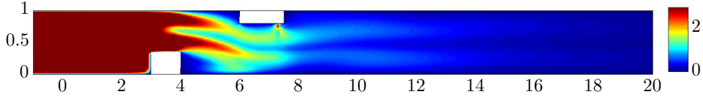
FIGURE 14. Controlled perturbation norm (case A)
