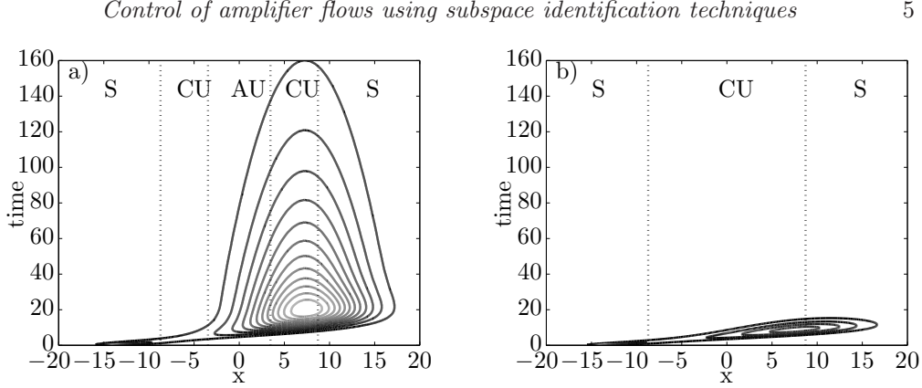
FIGURE 1. Response to an impulse from the noise location shown as |q| -contours in an x - t -diagram; (a) for a moderate convection speed U_r = 2 and (b) for a large convection speed U_r = 3 . Symbols denote the absolutely unstable (AU), convectively unstable (CU) or stable (S) spatial domains.
