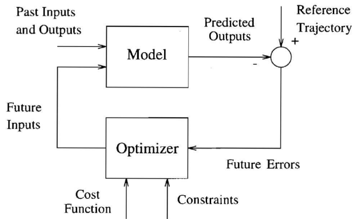
Figure 1.5: Schematic structure of a Model Predictive Controller, Camacho & Bordons (1999).
