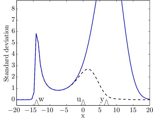
FIGURE 8. Standard deviation of the estimation error (dashed line) as a function of streamwise position x and standard deviation of the state (continuous line) as a function of x . For both curves, the convection speed is U_r = 3 .
