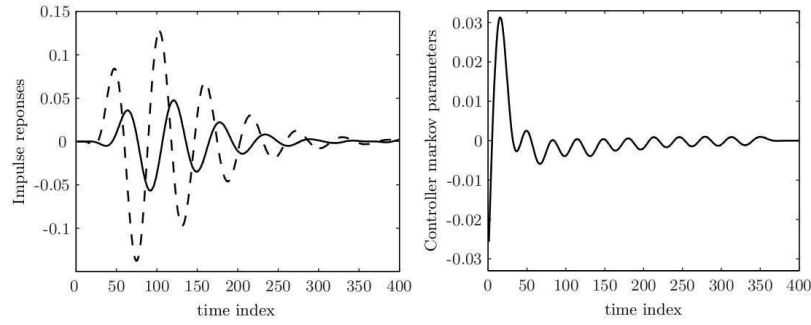
FIGURE 3. Left: Identified impulses responses, G_{uy} (dashed) and G_{uy}G_{ws}^{-1} (plain). Right: computed impulse response of the controller C_{su}
