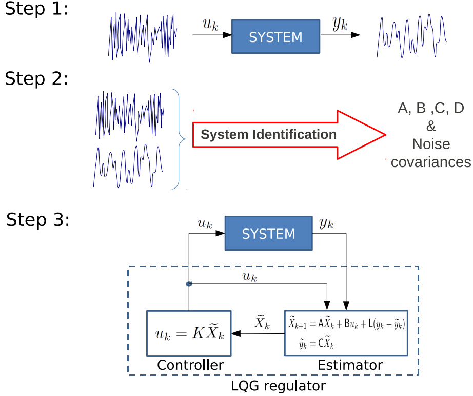
FIGURE 4. Procedural steps of control design based on system identification. Step 1: excitation of the system with a known input signal and simultaneous measurement of the output. Step 2: subspace identification of the model. Step 3: design of the LQG regulator and compensation of the system.
