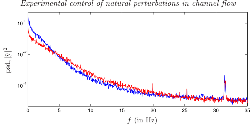
FIGURE 9. Power spectral density of the downstream (objective) sensor signal (blue) without control and (red) with control.
