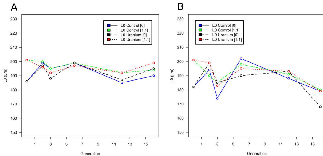
Figure VIII.4: Male (A) and hermaphrodite (B) hatching length L_0 ( \mu\text{m} ) for individuals issued from MGC (Control population) and MGU (Uranium population) exposed to control conditions or 1.1 mM U, as a function of the generation. Each point represents the L_0 value of the model (Eq. VIII.1) fitted using all the replicates for each treatment. L_0 Control [0] represents hatching length for MGC exposed to control conditions, L_0 Control [1.1] represents hatching length for MGC exposed to 1.1 mM U, L_0 Uranium [0] represents hatching length for MGU exposed to control conditions, and L_0 Uranium [1.1] represents hatching length for MGU exposed to 1.1 mM U.
