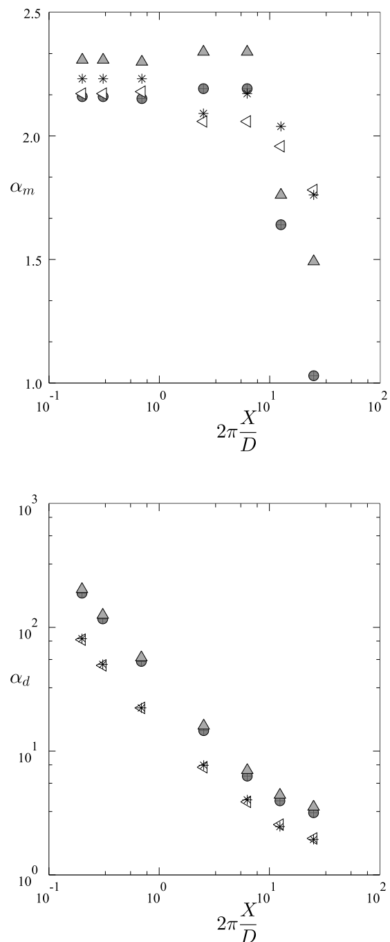
Fig. 8: mass and drag coefficients vs. Keulegan Carpenter number. \blacktriangle : center cylinder, \bullet : left central cylinder, \triangle : central upper cylinder, * : upper left cylinder
