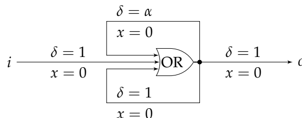
Figure 8.6: Circuit C_{ev} solving eventual SPF
