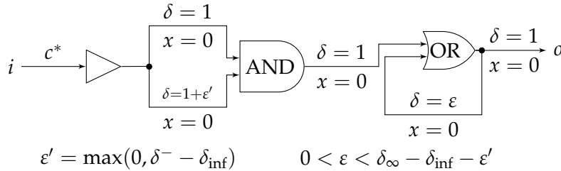
Figure 9.6: Circuit C_{NC} used in Case 2.2
