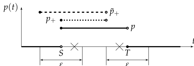
Figure 8.4: Input pulse p , together with its derived pulses p_+ and \tilde{p}_+ , and measure points for time \tilde{t}
