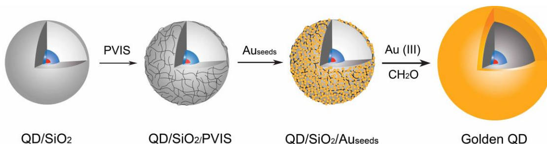
Figure 3.2. Scheme of the different steps leading from QD/SiO 2 to golden QDs (Au-shell-encapsulated QDs); PVIS: poly(1-vinylimidazole-co-vinyltrimethoxysilane).
