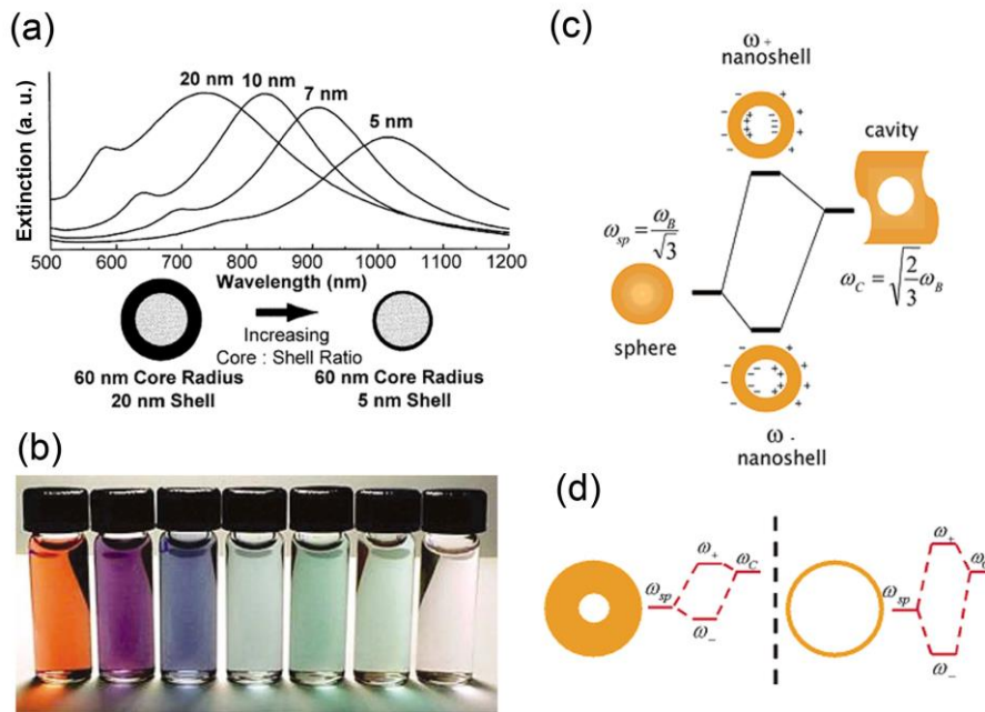
Figure 1.3: (a) Theoretically calculated optical resonances of Au nanoshells as a function of the ratio between the silica core radius and the Au shell thickness. (b) A photograph of aqueous dispersions of Au nanoshells with different frequencies of plasmonic resonances. (c) Plasmon hybridization in metallic nanoshells arises from the interaction between cavity plasmons and sphere plasmons. (d) The strength of the interaction between the sphere and cavity plasmons is dependent on the thickness of the shell. Reprinted from Ref [23, 25].
