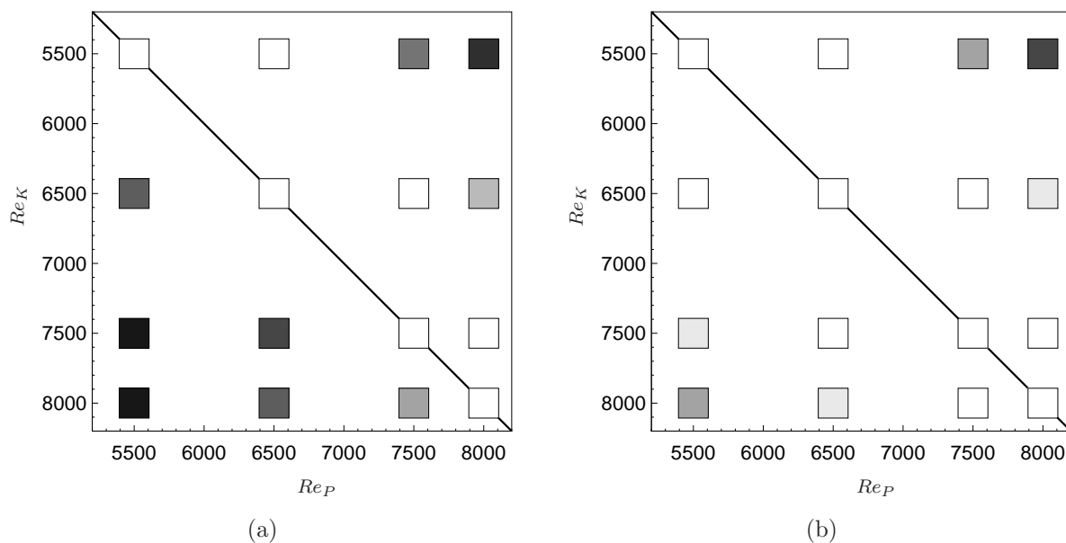
Figure 4.20: Stability behavior of \mathcal{H}_2 controllers, LQG/SGL (a) and LQG/LTR (b) at different Reynolds number. White squares represent maximum closed-loop poles with negative real parts (stable cases). Squares in gray scale represent maximum closed-loop poles with positive real parts (unstable). Instability intensity is represented through the color map from light gray (weak instability) to black (strong instability). Black solid line is the design locus, stable by definition since the plant P(s) and the compensator K(s) are obtained at the same Reynolds number ( Re_P and Re_K respectively).
