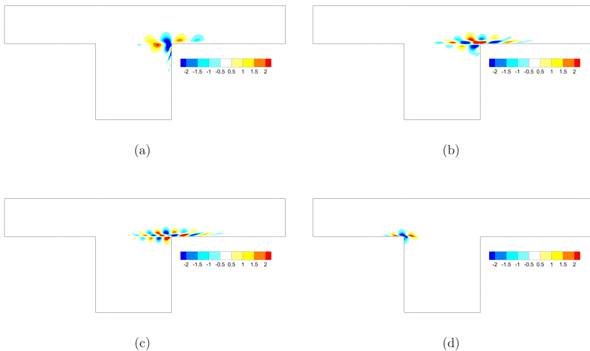
Figure 4.3: (a) cross-stream component of the direct global mode at \omega = 7.9 ; (b) streamwise component of the direct global mode at \omega = 10.9 ; (c) streamwise component of the direct global mode at \omega = 16.7 ; (d) cross-stream component of the adjoint global mode at \omega = -13.8 .
