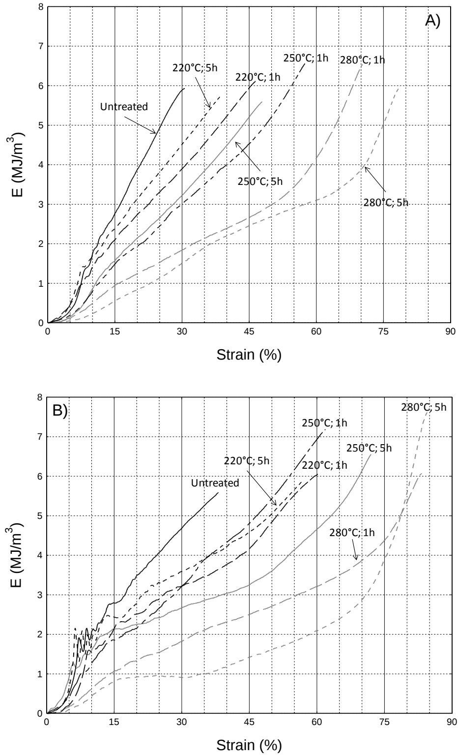
Figure IV-11. Absorbed energy versus deformation for maritime pine (A: radial compression; B: tangential compression).
