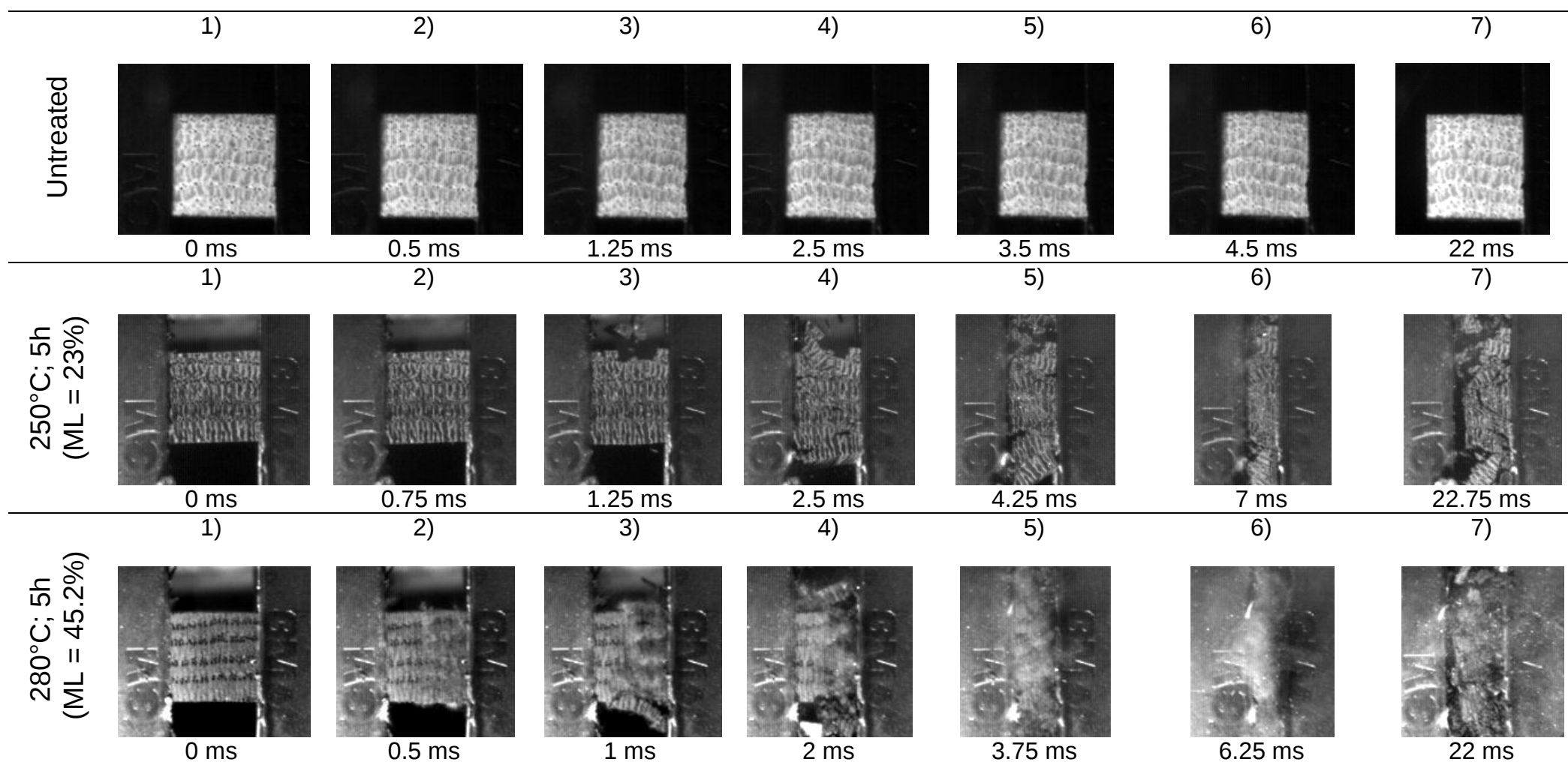
Figure IV-5. Deformation of untreated and heat treated pedunculate oak during dynamic compression (tangential direction).
