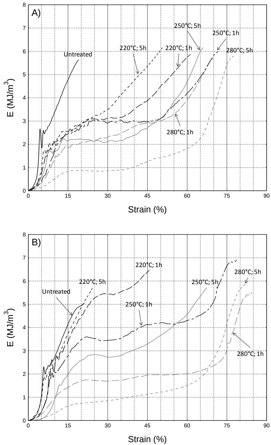
Figure IV-12. Absorbed energy versus deformation for pedunculate oak (A: radial compression; B: tangential compression).
