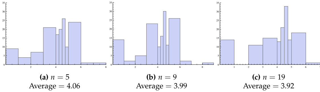
Figure 6.4.1. The global histograms of the cutoff strategies for each phase within Sessions 1 – 7. Hence we have, in total, 140 observations for each case where the payoffs are 900 : 200. Note that the intervals [4, 5) , which are the most voluminous, are divided into four equal subintervals.
