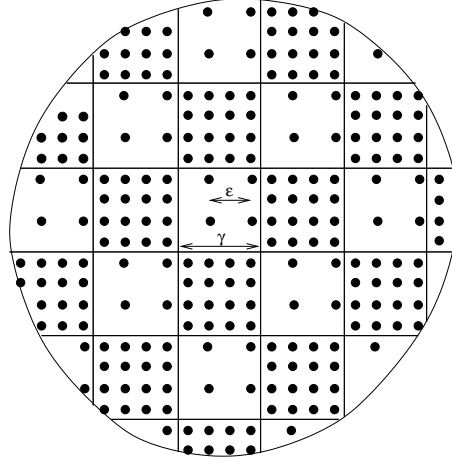
Figure 3: The limiting process allowing to derive (76), with K = 2 .
