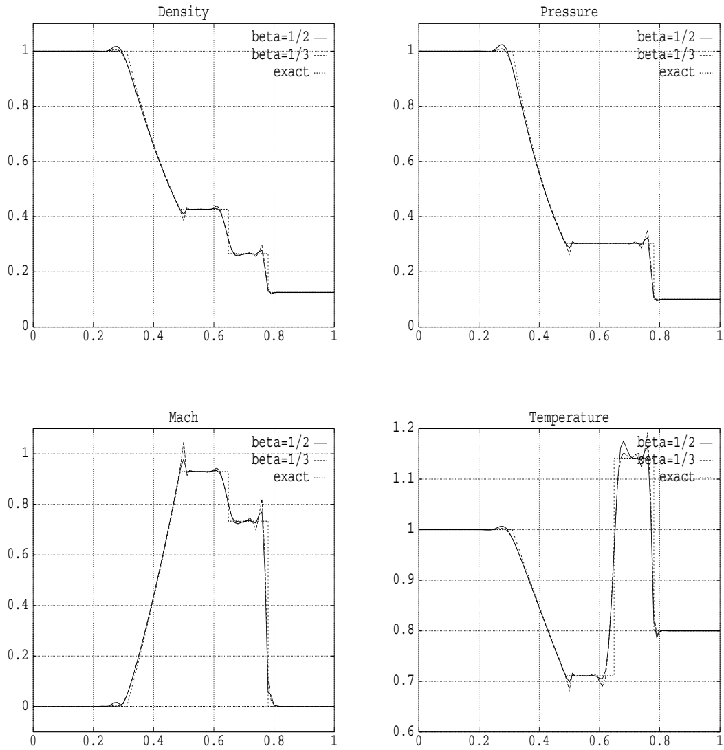
FIG. VII.7 – Shock tube solutions with no limitation.
