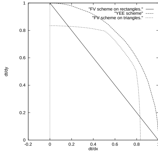
FIG. III.3 – Stability domains for Yee and first-order finite volume schemes.
