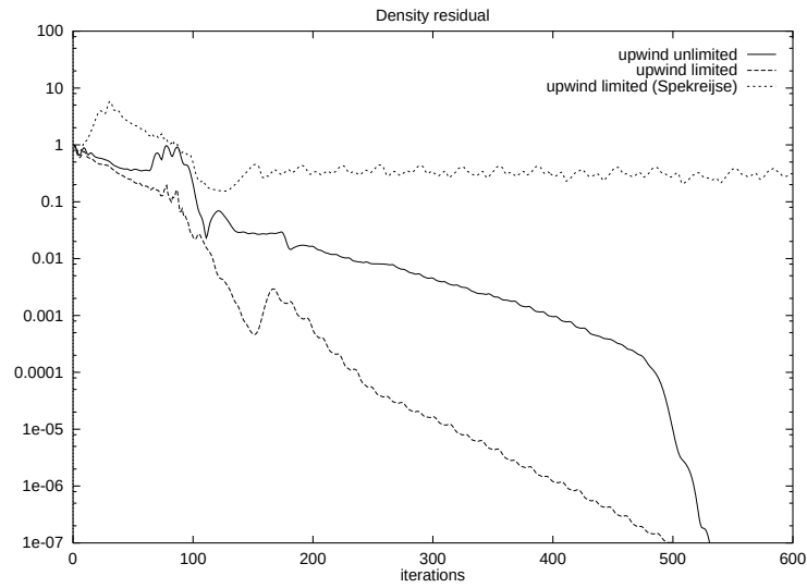
FIG. VII.14 – L^2 -norm residual of the density through iterations (2280 vertices).
