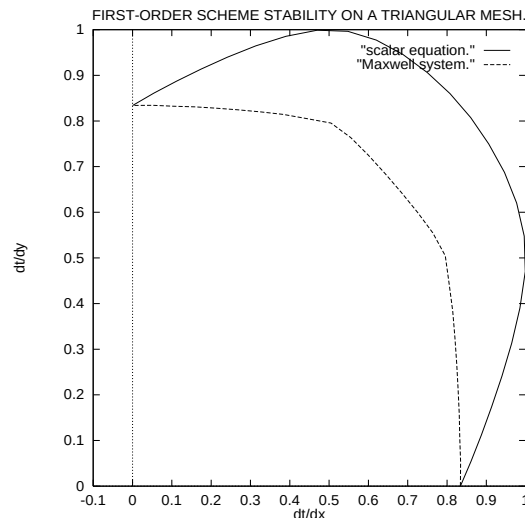
FIG. III.2 – Maxwell system and convection equation.
