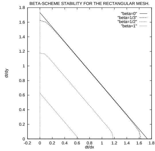
FIG. III.5 – Convection equation.
