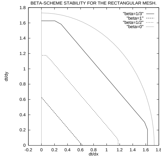
FIG. III.4 – Maxwell system.
