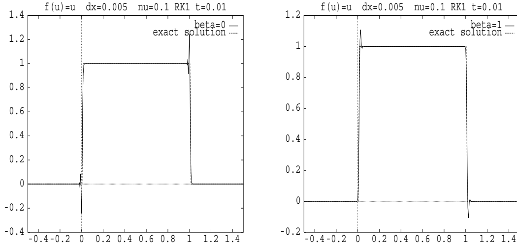
FIG. VII.2 – Spurious oscillations for \beta = 0 and \beta = 1 .
