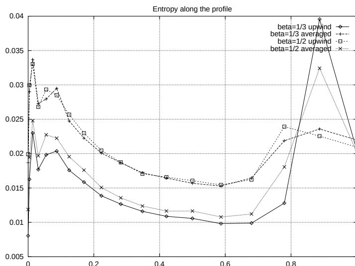
FIG. VII.12 – Entropy along the profile for different gradients and MUSCL limited schemes (800 vertices).
