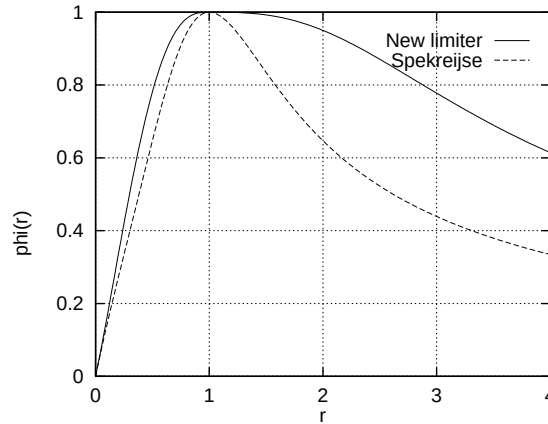
FIG. VII.3 – The new limiter function compared with Spekreijse's.
