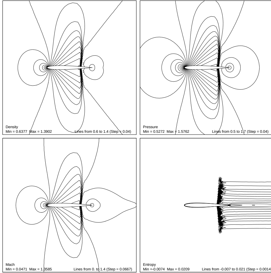
FIG. VII.16 – Density, pressure, Mach and entropy contours for the steady solution with \beta = 1/3 and the new limiter (12214 vertices).
