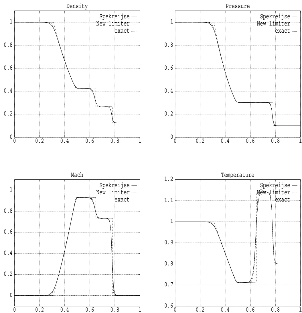
FIG. VII.8 – Third-order shock tube solutions.
