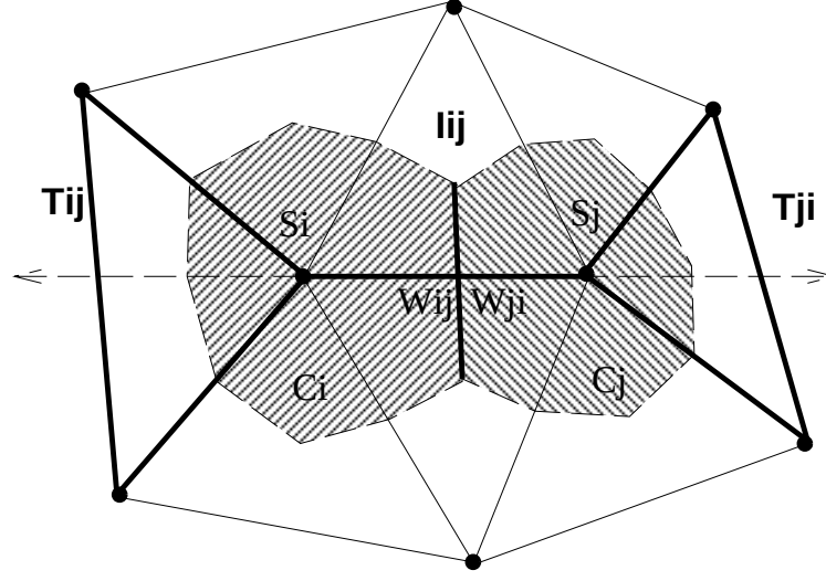
FIG. VII.6 – MUSCL extension in two dimensions, and upwind and downwind triangles.
