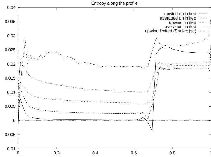
FIG. VII.13 – Profile entropy for different gradients and limiters (2280 vertices).
