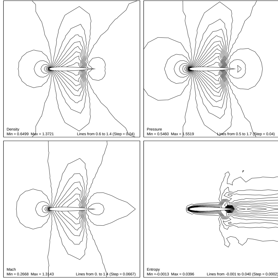
FIG. VII.11 – Density, pressure, Mach and entropy contours for the steady solution with \beta = 1/3 and the new limiter (800 vertices).
