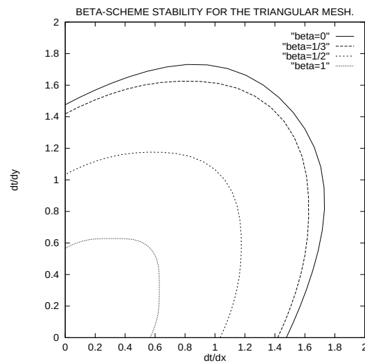
FIG. III.7 – Convection equation.
