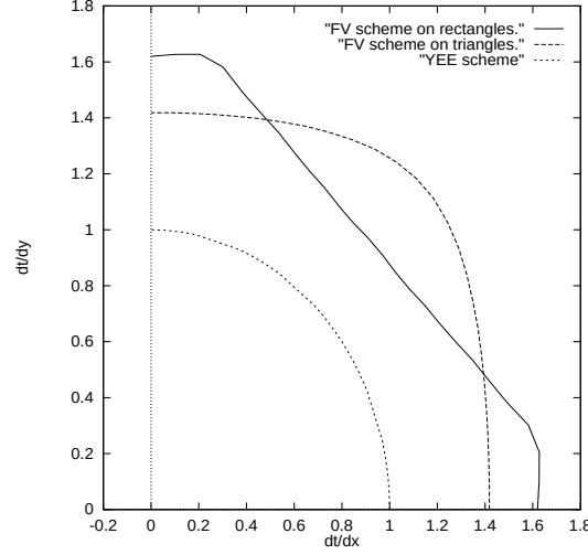
FIG. III.8 – Stability domains for Yee and third-order finite volume schemes.
