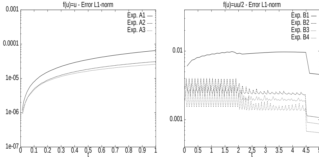
FIG. VII.5 – Error L_1 -norm for hyperbolic equations simulations.
