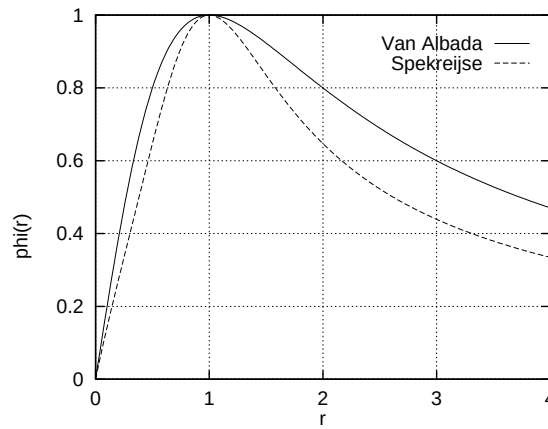
FIG. VII.1 – Limiter functions: Van Albada's average and Spekreijse's.
