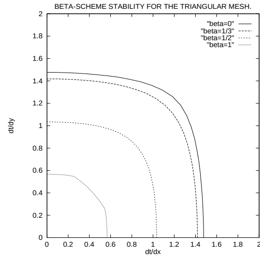
FIG. III.6 – Maxwell system.
