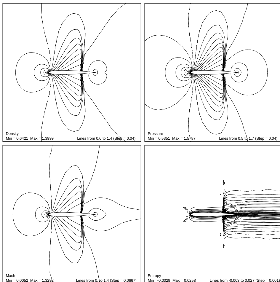
FIG. VII.15 – Density, pressure, Mach and entropy contours for the steady solution with \beta = 1/3 and the new limiter (2280 vertices).
