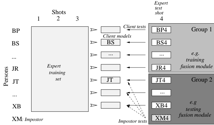
Figure 8.1: Visualization of the leave-one-out validation protocol.
