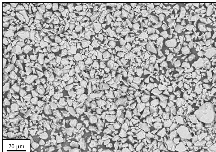
a) Poudre \text{Al}_2\text{O}_3 [-12 +2 µm]
