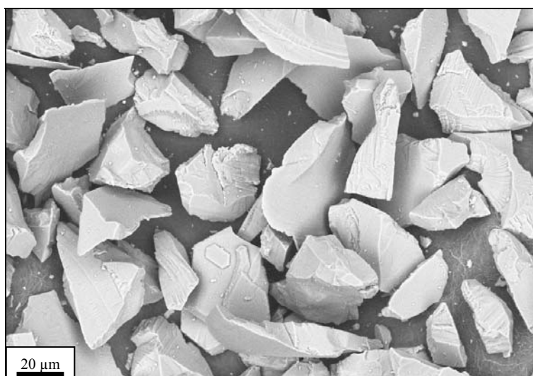
c) Poudre \text{Al}_2\text{O}_3 [-70 +20 µm]
