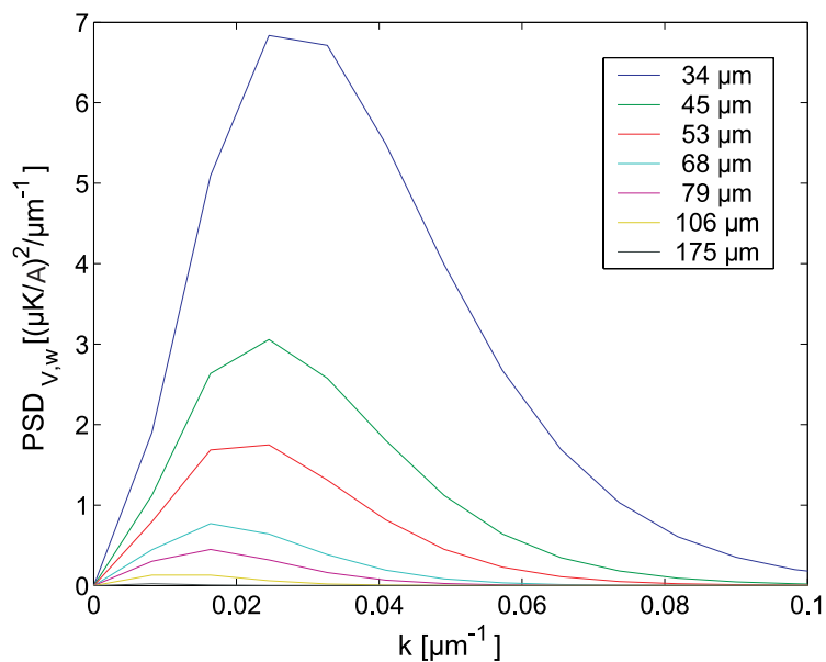
Figure 6.13: Power spectral density of the roughness potential as calculated from the power spectral density of the border of the wire for different heights as given in the graph.
