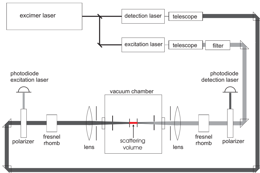
Figure 2.2: Layout of the optical components.
