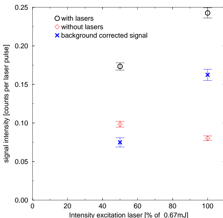
Figure 2.18: Signal of CaAr optical collision for two intensities of the excitation laser. Detuning: 300\text{ cm}^{-1} , scattering angle: 21.6^\circ . The background signal is measured by turning off the lasers.
