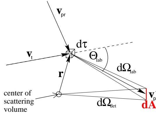
Figure 2.24: Illustration of the differential scattering rate.
