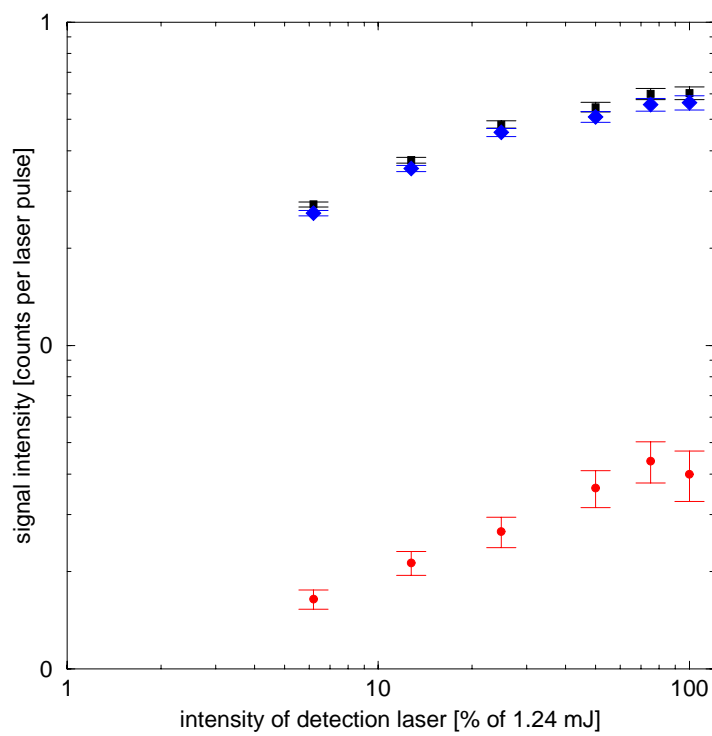
Figure 2.22: Signal dependency on detection laser intensity: High intensities. Detuning: 480 \text{ cm}^{-1} , scattering angle: 21.6^\circ
