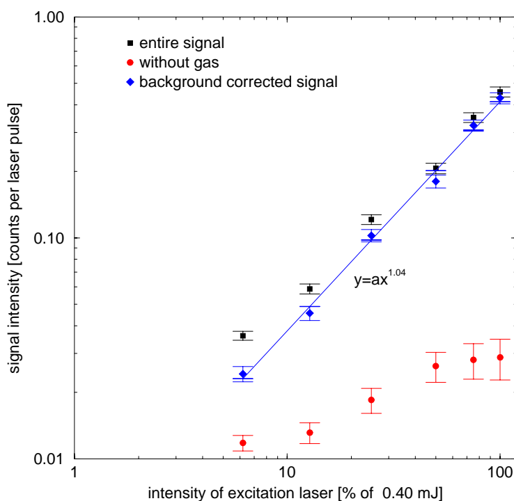
Figure 2.20: Signal dependency on intensity of excitation laser. Detuning is 480\text{ cm}^{-1} , scattering angle 21.6^\circ .
