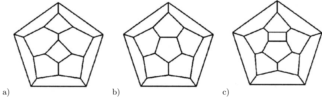
Figure I.28 : Schlegel diagrams : a) combination 2-8-2, b) combination 0-12-0, c) combination 1-10-2.
