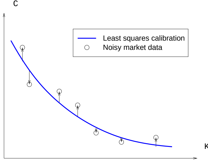
Figure 3.3: Estimating the noise level in the data.
