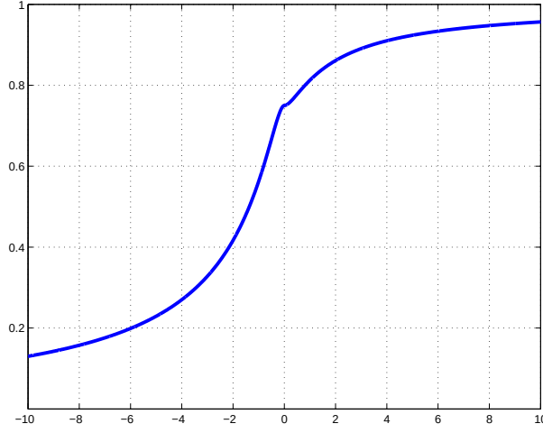
Figure 5.3: Conditional distribution function F_\xi , corresponding to the Lévy copula of Example 5.1 with \xi = 1 , \theta = 1 and \eta = 0.25 .
