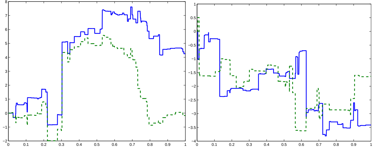
Figure 5.4: Trajectories of two variance gamma processes with dependence structure given by the Lévy copula of Example 5.1. In both graphs both variance gamma processes are driftless and have parameters c = 10 , \lambda_- = 1 and \lambda_+ = 1 (cf. Equation (1.19)). In the left graph, the dependence between the two components is strong both in terms of sign and absolute value ( \eta = 0.9 and \theta = 3 ): the processes jump mostly in the same direction and the sizes of jumps are similar. In the right graph the dependence of absolute values is weak ( \theta = 0.5 ) and the dependence of jump sign is negative ( \eta = 0.25 ).
