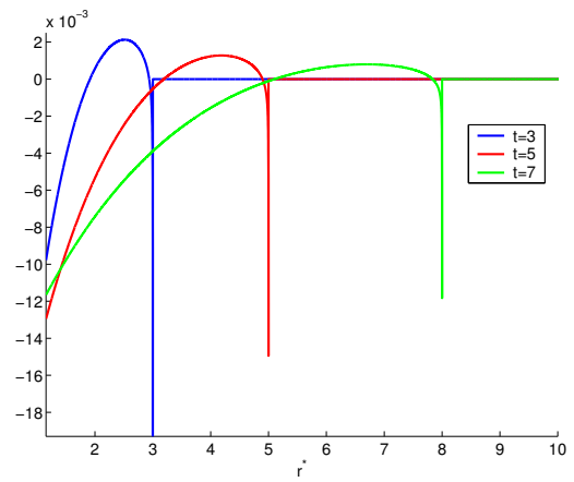
FIG. 8.24: t \mapsto G_r^2(\mathbf{x}, t), \theta = \pi/6
