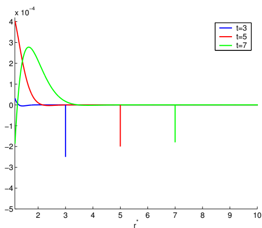
FIG. 8.26: t \mapsto G_r^{10}(\mathbf{x}, t) , \theta = \pi/6
