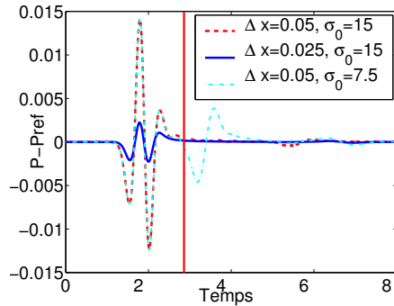
FIG. 11.7: P - P_{ref}
