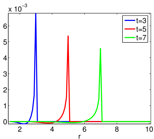
FIG. 9.28: r^* \mapsto \gamma_r^{\sigma,50}(r^*, \theta = \pi/6, t)
