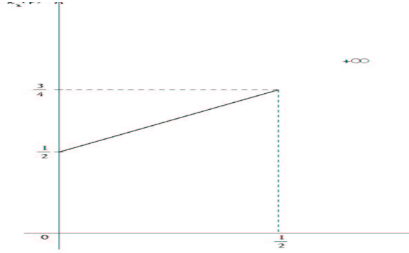
FIG. 4.4 – 2-microlocal spectra of the Riemann Function on R_{3/2} (left), R_{1/2} (middle) and S_\tau (right).
