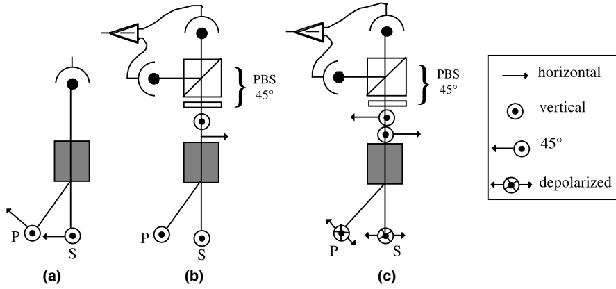
Fig. 1. Implemented architectures, (a) direct detection, (b) anisotropic diffraction; (c) depolarized configuration. Both beams enter by the (110) faces and the grating vector is along (110).
