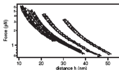
FIG. 1. Force-distance profile of the particles grafted with streptavidin, C_p = 0.05\% volume in pH 7.2 phosphate buffer as a function of the ionic strength. \circ : 1 mM ( \kappa^{-1} = 9.5 nm), \square : 2 mM ( \kappa^{-1} = 6.7 nm), \triangle : 5 mM ( \kappa^{-1} = 4.2 nm), + : 10 mM ( \kappa^{-1} = 3 nm), \diamond : 20 mM ( \kappa^{-1} = 2.1 nm). The surface to surface separation h is deduced from: h = d - 2R . The distance d is measured from Bragg scattering and 2R is the hard core diameter. Plain lines give the confidence interval for the calculated profiles, taking into account an error of 1 nm on the distance measured. To measure R , the particles were pushed to contact in a solution of 10 mM chlorhydric acid for which the COOH functions present at the surface of the particles are completely protonated. The evolution of the repulsive profiles with ionic strength shows that both electrostatic and steric forces help to stabilize the particles.
