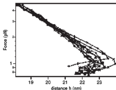
FIG. 3. Force-distance profiles in the presence of 1.9 DNA on average between adjacent particles, in phosphate buffer 10 mM pH 7.2. \bullet : increasing field ramps, \times : decreasing field ramps, \blacktriangle : average force-distance profile. Dashed lines are guides to the eye.
