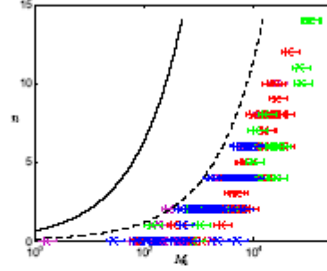
FIGURE 4. Test of linear dynamics as a predictor for the formation of arches. The sequence of applied fields is described in the text and filaments of lengths ranging from 10\text{ }\mu\text{m} up to 150\text{ }\mu\text{m} , are constructed from particles of diameter 2a = 750\text{ nm} supplied by Ademtech and linked by polyacrylic acid, with a bending stiffness of K_b = (6.3 \pm 2.3) \times 10^{-24}\text{ Jm} , and susceptibility \chi = 1.62 . Different coloured data-sets correspond to different field strengths: B_c = \sqrt{B_t^2 + B_z^2} = 6.21\text{ mT} (magenta); B_c = 8.97\text{ mT} (blue); B_c = 12.44\text{ mT} (red) and B_c = 17.80\text{ mT} (green). The error bars reflect uncertainty in bending stiffness. The solid curve represents the lower bound derived in §3.1 based on linear dynamics, and the dashed curve the criterion ( m_n > 75 ) postulated in §3.2 on stability grounds.
