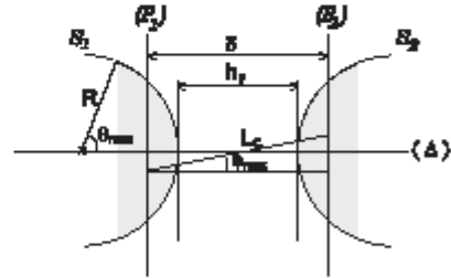
FIG. 5. Definition of the different geometrical parameters appearing in the model. The angle \theta_{\max} defines the reactive portion of sphere and the distance h_f is the distance between the particles during the linking process (formation of permanent chains): \cos\theta_{\max} = (h_f + 2R - L_c)/2R . L_c = 51 nm is the contour length of the DNA and R = 88 nm is the radius of the particles. \delta is the distance between the planes (P_1) and (P_2) that are used for approximation. \varphi_{\max} defines the maximal orientation that can take a DNA molecule when linking the beads. The figure is invariant by rotation around (\Delta) , the axis of the chain.
