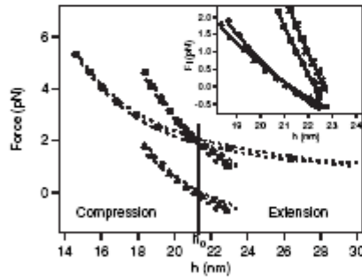
FIG. 4. Comparison between average force-distance profiles in the absence and in the presence of 1.9 DNA on average between adjacent particles, in phosphate buffer 10 mM pH 7.2: ●: F_{B_0} , ■: F_{B_1} , ▲: F_l = F_{B_1} - F_{B_0} . Dashed lines correspond to the error on force-distance profiles, calculated from the standard deviation of the measured profiles. Inset: contribution of the linker F_l and fit of the data for various numbers of DNA between the particles. ▲: 1.9 DNA, ◊: 3 DNA, □: 4.7 DNA, ×: 5.5 DNA. Plain lines: fit of the data with F_{B_1} = N(F)_\varphi , with N = 1.9 and (F)_\varphi given by Eq. (3).
