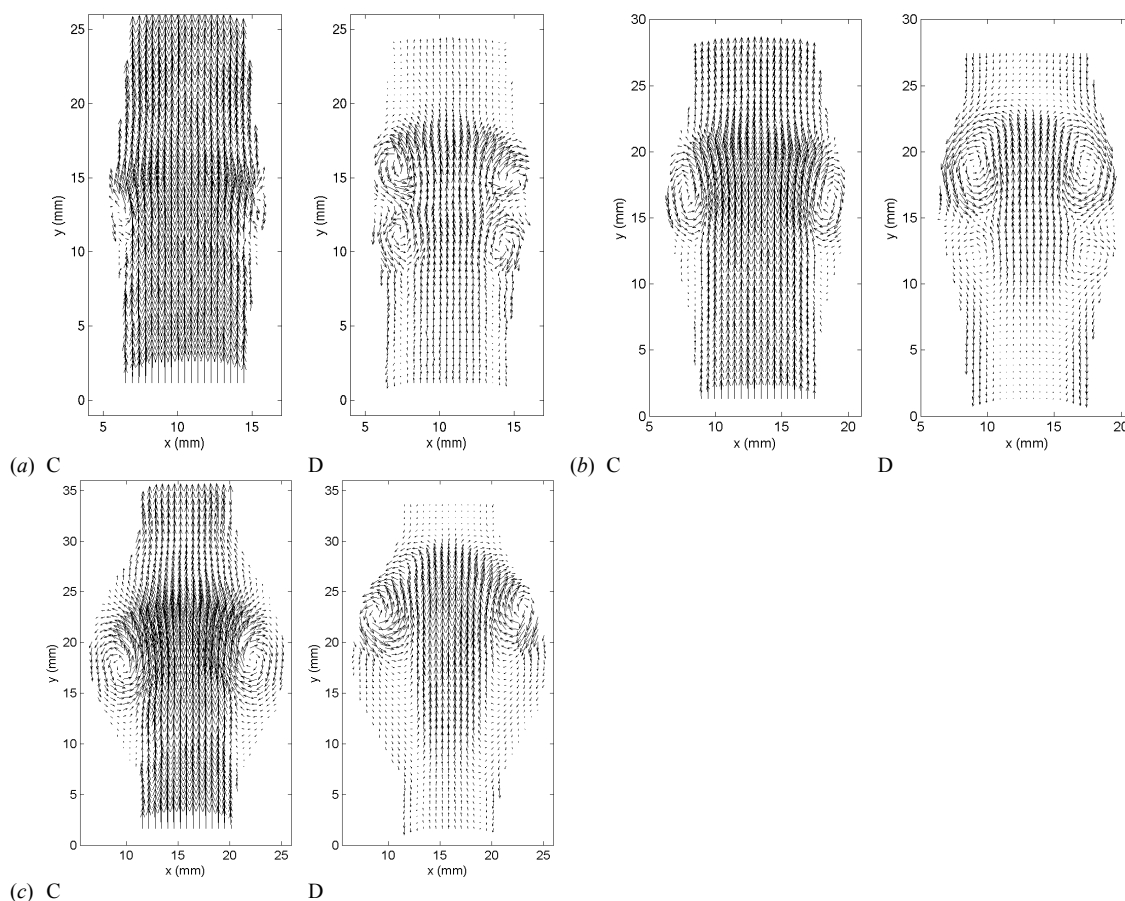
Figure 3.10: Comparison of the phase-averaged velocity field measured with the PIV system in models 1 – D/d = 1.3 (a), 2 – D/d = 1.5 (b) and 5 – D/d = 2.1 (c) at times C and D. A small phase-lag between the different experiments is possible, since the frequency
